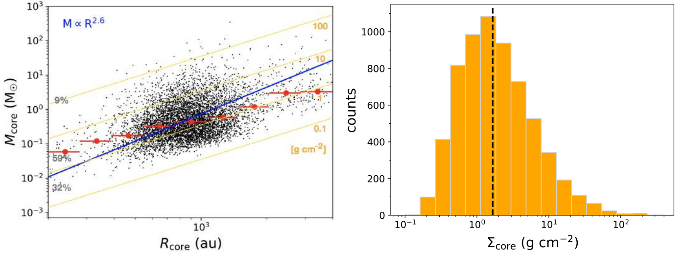
Fig. 17. Mass–radius relation and mass surface density distribution for the core sample. Left panel: core masses as a function of estimated radius. Solid gold lines represent different values of core surface density: from bottom to top, 0.1, 1, 10, and 100 \text{g cm}^{-2} , respectively. Percentages of data points within the corresponding bins of surface density are given in grey. Red points indicate the median M_{\text{core}} values in given bins (red bars) of R_{\text{core}} . The solid blue line is the best fit to the data points, corresponding to the power-law relation reported in the top-left corner. Right panel: distribution of the mass surface density of the cores. The vertical dashed black line marks the median value of 1.7 \text{ g cm}^{-2} .
