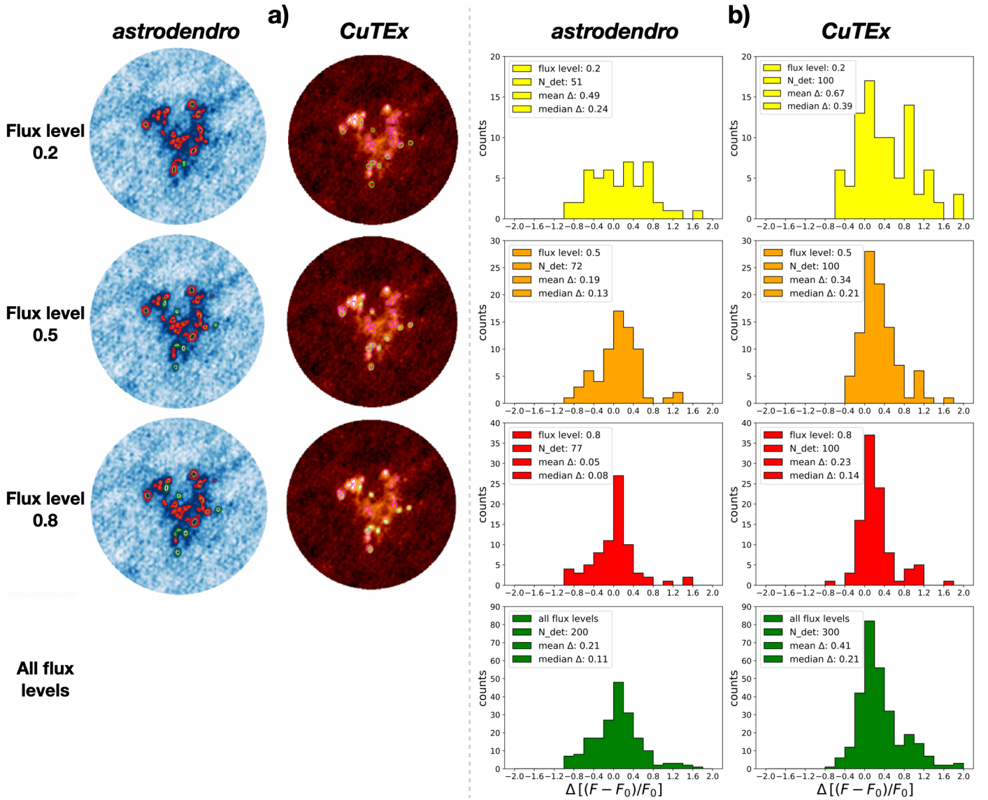
Fig. A.1. Comparison of the outcome of the source extraction tests performed with astro dendro and CuTEX . a) Comparison of the detections obtained with astro dendro (left column panels) and CuTEX (right column panels) on the continuum map of the ALMAGAL field AG304.5567+0.3273 added with 10 synthetic sources with three different flux levels (see text for details). The three flux levels reported to the side refer to fractions of the native map peak flux. Green contours/ellipses mark the detected sources that were matched with the truth tables from the simulation code (i.e., the recovered synthetic sources), while red/magenta contours/ellipses indicate detected but unmatched sources. b) Comparison of the outcome of the photometry procedure performed with the implemented version of astro dendro (left column panels) and CuTEX (right column panels) on the set of simulated maps (see text for details). In detail, histograms of the relative discrepancies (referred to as \Delta ) between measured integrated fluxes ( F ) and generated ones ( F_0 ) are shown for the matched synthetic sources detected at each flux level (100 injected sources in total, first three rows) and for all flux levels combined (300 injected sources in total, last row). Boxes within individual panels report the corresponding number of detections and the mean and median values of the relative discrepancy in the flux.
