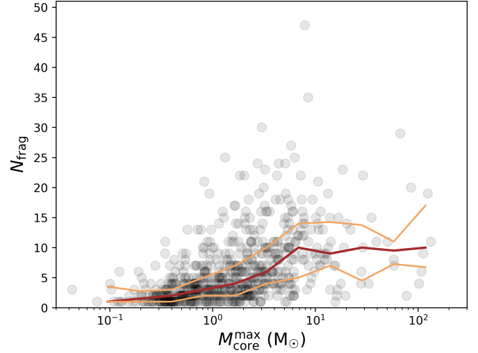
Fig. 20. Number of detected compact fragments (cores) as a function of M_{\text{core}}^{\text{max}} for each clump. Points are drawn in transparency to highlight the local density of the data. The solid brown line draws the trend of the median N_{\text{frag}} in given bins of M_{\text{core}}^{\text{max}} . The solid lighter brown lines correspond to the 25th (bottom) and 75th (top) percentiles of the N_{\text{frag}} distribution within the same bins.
