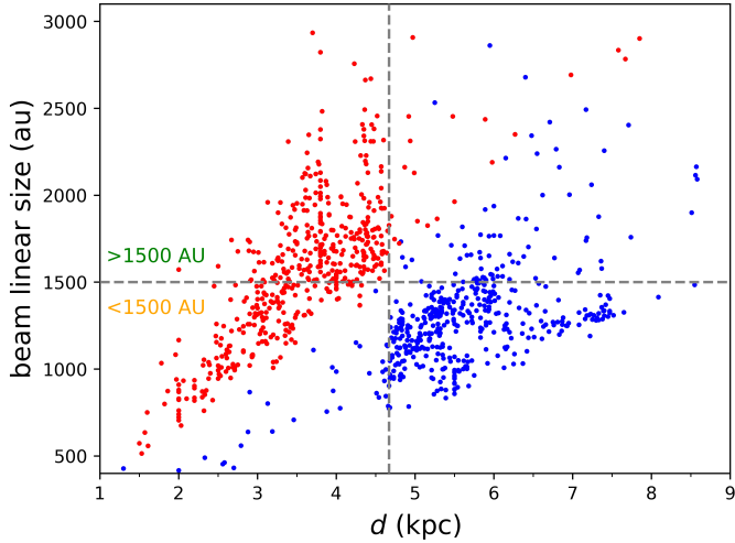
Fig. 2. Linear size of the map beam as a function of the heliocentric distance of the ALMAGAL clumps. Targets observed with near or far sample configurations appear as red or blue points, respectively. The vertical dashed grey line marks the nominal \sim 4.7 kpc distance limit separating the near and far subsamples (with the few exceptions described in Sect. 2.3). The horizontal dashed grey line separates higher spatial resolution fields (i.e., beam linear size < 1500 au) from lower resolution ones ( > 1500 au). Note: for better visualization purposes, distance and/or resolution outliers are not shown in this plot ( \sim 30 targets, \leq 3\% ).
