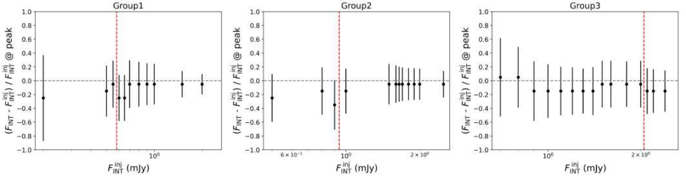
Fig. B.1. Photometric accuracy analysis: source integrated fluxes. Peak value (the mode) of the distribution of the relative discrepancy between measured ( F_{\text{INT}} ) and simulated ( F_{\text{INT}}^{\text{inj}} ) integrated fluxes, as a function of the injected flux level F_{\text{INT}}^{\text{inj}} (Group 1 left panel, Group 2 middle panel, Group 3 right panel). In all panels, the vertical error bars mark the interquartile range of the distribution within each level, while the vertical dashed red line reports the estimated flux completeness limit for the current group. The horizontal dashed grey line marks the equality between F_{\text{INT}} and F_{\text{INT}}^{\text{inj}} .
