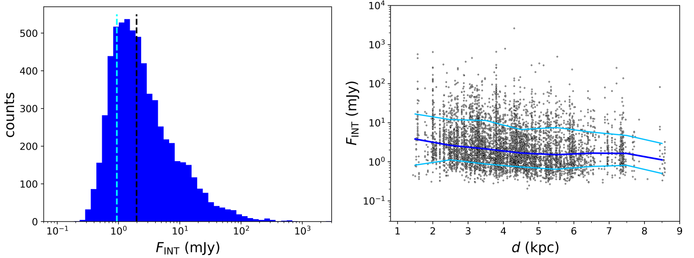
Fig. 11. Integrated fluxes of the extracted compact sources as estimated with CuTE . Left panel: overall distribution of the integrated fluxes of the sources. The adopted flux completeness value of 0.94 mJy (see Sect. 3.3) is marked by the vertical dashed cyan line. The vertical dashed black line marks the median value of the distribution (2 mJy). Right panel: measured integrated fluxes of the sources as a function of the hosting clump distance. The solid blue line traces the median F_{\text{INT}} values within given bins of distance. Light blue lines correspond to the 15th (bottom) and 85th (top) percentiles of the flux distribution in the same bins of distance. Note: for improved visualization, distance outliers (<3%) are not shown in this plot.
