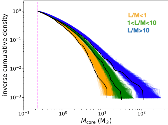
Fig. 18. Observed CMFs (black lines, expressed as inverse cumulative number density distributions) for the three populations of ALMAGAL cores classified, as reported, according to the L/M evolutionary indicator of the hosting clump, as explained in Sect. 5.2.1. The three colored bands trace, for each population, the 1000 MC realizations of CMFs computed by assigning to each core a random temperature within the ranges defined in Table 6. Less evolved sources (i.e., with L/M \leq 1 L_{\odot}/M_{\odot} ) are marked by golden lines, the intermediate ones ( 1 < L/M \leq 10 L_{\odot}/M_{\odot} ) by green lines, and the more evolved sources ( L/M > 10 L_{\odot}/M_{\odot} ) by blue lines. Note: we include only cores above the mass completeness value of 0.23 M_{\odot} , marked by the vertical dashed magenta line (see text for explanation).
