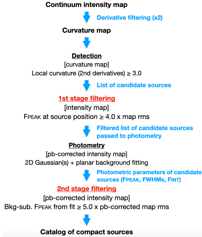
Fig. 4. Diagram of the main phases of the source detection and photometry pipeline developed and used in this work. Underlined black steps were already present in the original CuTE x version (but were still further implemented in this work), while those in red have been newly introduced in the context of the present work.
