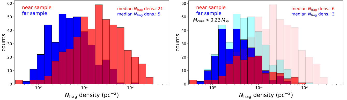
Fig. 10. Analysis of the derived spatial density of the cores. Left panel: distribution of the spatial density of the cores within each clump for near sample (red bars) and far sample (blue bars) sources, respectively. Right panel: same as left panel, but only including clumps containing core masses above 0.23 M_{\odot} . For comparison, the overall distributions of the left panel appear here in transparency in the background as pink (near sample) and cyan (far sample) bars, respectively. In both panels, overlapping areas between the two distributions are marked by the magenta bars. The median values of the near and far sample distributions are also reported in each panel.
