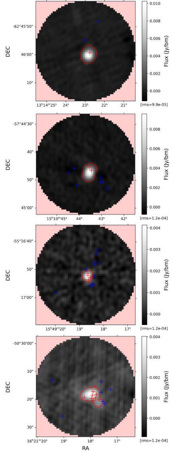
Fig. D.1. Cutouts of CORNISH/CORNISH-South radio continuum emission maps (5 GHz frequency, \sim 1'' angular resolution) corresponding to the ALMAGAL fields (from top to bottom): AG305.5535-0.0114 (first panel), AG320.6753+0.2459 (second panel), AG326.4486-0.7484 (third panel), and AG333.2217-0.4020 (fourth panel). Red contour levels indicate 7\sigma_{\text{rms}}^{\text{rad}} emission regions. Red crosses mark the locations of the ALMAGAL cores that fell within such radio emission contours and are thus considered as potentially contaminated, whereas blue crosses mark the unmatched ALMAGAL cores.
