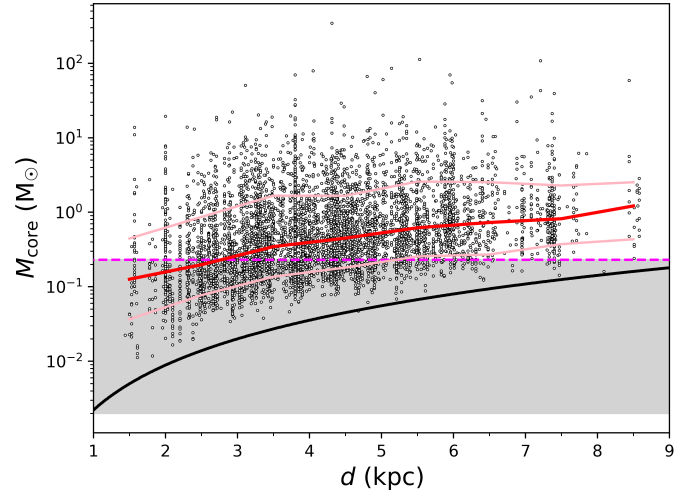
Fig. 16. Estimated core masses as a function of the hosting clump heliocentric distance, highlighting the variation of mass sensitivity across distance. The red line draws the trend of the median value among core masses contained within 1 kpc bins of distance, and the two pink lines mark the position of the 15th (bottom) and 85th (top) percentiles of the mass distribution within the same distance bins. The horizontal dashed magenta line marks the mass completeness limit of 0.23 M_{\odot} , while the solid black curve is drawn to approximately follow the trend of the minimum core mass revealed with target distance. The grey shaded area highlights the incomplete part of the sample, and, in particular, the region below the black curve represents the “forbidden” (i.e., not detectable) range of masses based on revealed objects at the different target distances. Note: for better visualization purposes, distance outliers ( <3\% ) are not shown in this plot.
