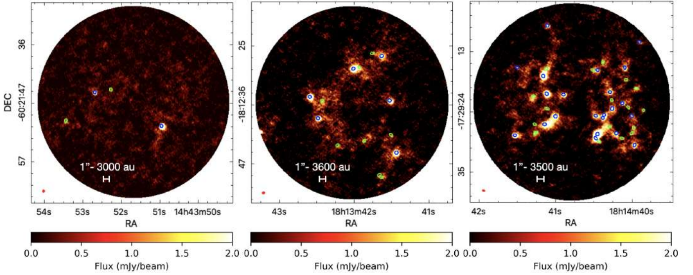
Fig. 6. Outcome of the source extraction procedure performed with CuTE x on selected ALMAGAL clumps (from left to right, fields AG316.4045-0.4657, AG012.4977-0.2233, AG013.2428-0.0854). As in Fig. 5, the blue ellipses mark the compact sources detected at 5\sigma_{\text{rms}} . The three clumps showcase the variety of fragmentation degree, morphologies of structures and patterns of emission revealed across the ALMAGAL sample. The CuTE x algorithm was optimized and tested in order to efficiently perform in all these different conditions. The green ellipses mark the sources that are recovered by allowing a signal-to-noise ratio (S/N) cut of 3\sigma_{\text{rms}} . The map beam is reported in red in the bottom-left corner of each panel.
