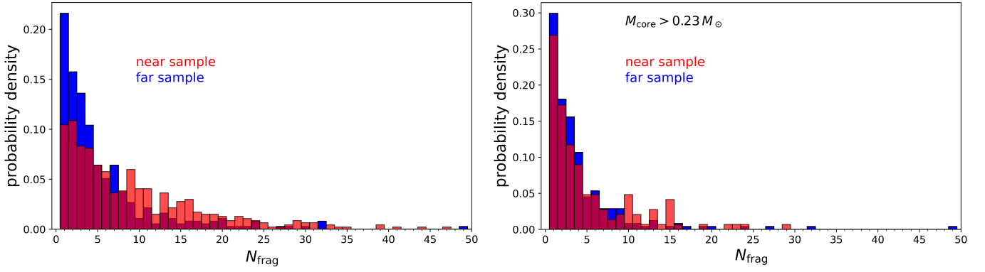
Fig. 9. Fragmentation statistics evaluated for near sample and far sample sources separately. Left panel: probability density distribution of the number of cores detected in each clump for near sample (red bars) and far sample (blue bars) sources, respectively. Right panel: same as left panel, but only including clumps containing core masses above 0.23 M_{\odot} (see text for interpretation). Detailed statistics for the individual distributions are reported in Table 5.
