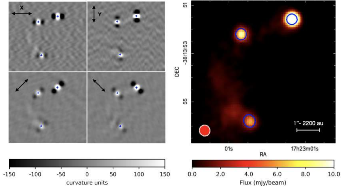
Fig. 5. Example of the source extraction procedure performed with CuTEs (see Fig. 4) for the ALMAGAL field AG349.6440-1.0948. Left panel: detection phase performed on curvature images along the reported four different directions; the blue crosses mark the candidate compact sources. Right panel: outcome of the photometry procedure performed on the corresponding intensity image; the blue ellipses represent the estimated shape of the compact sources (in terms of FWHMs and position angle, \lambda_{PA} ) as a result of the 2D Gaussian fitting procedure (see Sect. 3.2 for details). Note: the color scale of the image was adjusted to highlight all the three sources at the same time, so their visual appearance in terms of emission extent might not correspond to their actual size (ellipses). The map beam is shown in red in the bottom-left corner of the plot. The angular and physical scales are also reported.
