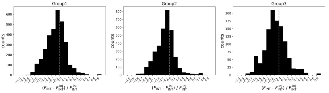
Fig. B.2. Photometric accuracy analysis: source integrated fluxes. Flux relative discrepancy distribution aggregating all flux levels above the completeness limit of the group (Group 1 left panel, Group 2 middle panel, Group 3 right panel). The vertical dashed grey line marks the equality between F_{\text{INT}} and F_{\text{INT}}^{\text{inj}} .
