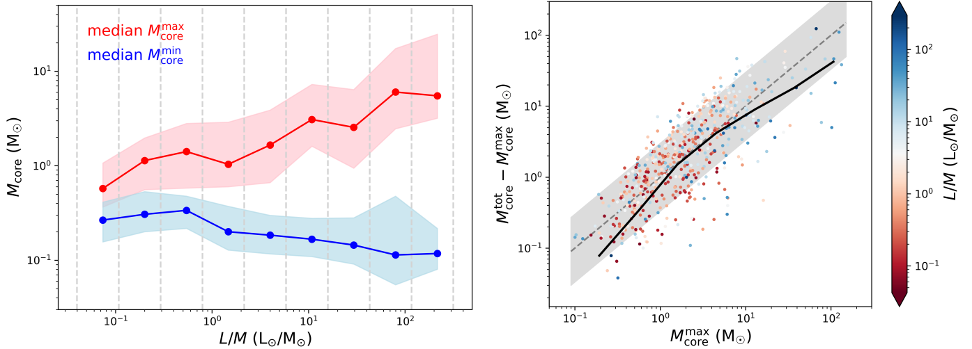
Fig. 19. Evolution of core masses. Left panel: median values of the maximum ( M_{\text{core}}^{\text{max}} , red) and the minimum ( M_{\text{core}}^{\text{min}} , blue) core masses revealed within different bins of clump L/M (delimited by vertical dashed grey lines). The respective colored shaded areas mark the 25th and 75th percentiles of the two distributions within the same L/M bins. Right panel: combined mass of the cores ( M_{\text{core}}^{\text{tot}} ) minus the mass of the MMC within each clump, as a function of the latter. Data points are color-coded by the clump L/M . The solid black line draws the trend of the median value of the quantity on the y -axis in given bins of M_{\text{core}}^{\text{max}} . The dashed grey line corresponds to the M_{\text{core}}^{\text{tot}} = 50\% M_{\text{core}}^{\text{max}} relation, while the shaded grey area marks (from top to bottom) the 25–75% range.
