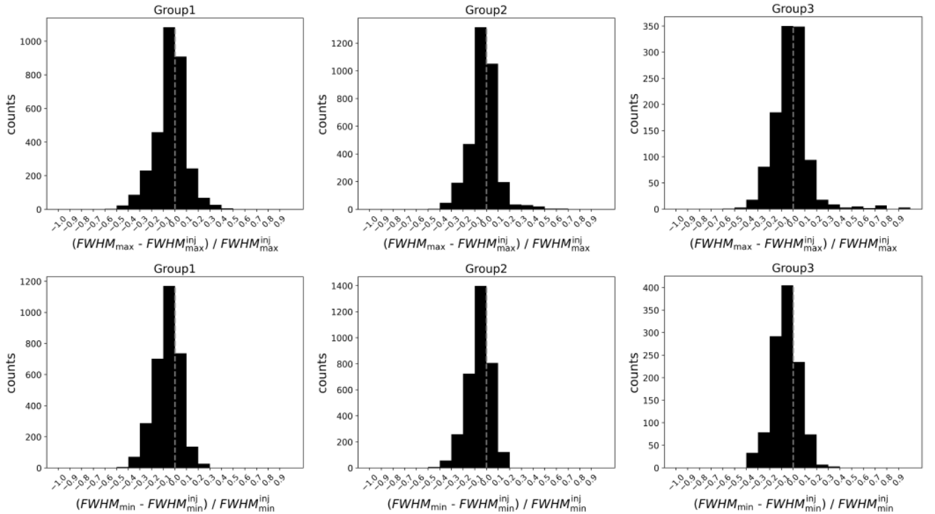
Fig. B.3. Photometric accuracy analysis: source angular sizes. Distribution of the relative discrepancy between measured ( FWHM ) and simulated ( FWHM^{\text{inj}} ) sizes, in terms of major (top row) and minor (bottom row) axes of the detected source ellipse (Group 1 left panels, Group 2 middle panels, Group 3 right panels). As in Fig. B.2, only flux levels above the completeness limit are considered for each group. In all panels, the vertical dashed grey line marks the equality between FWHM and FWHM^{\text{inj}} .
