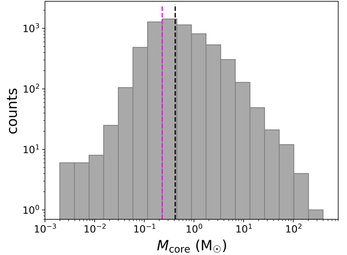
Fig. 15. Overall distribution of the estimated core masses. The vertical dashed magenta line marks the average mass completeness limit of 0.23 M_{\odot} estimated for our sample (see Sect. 5.2.4), while the vertical dashed black lines marks the median value of the distribution ( 0.4 M_{\odot} ).
