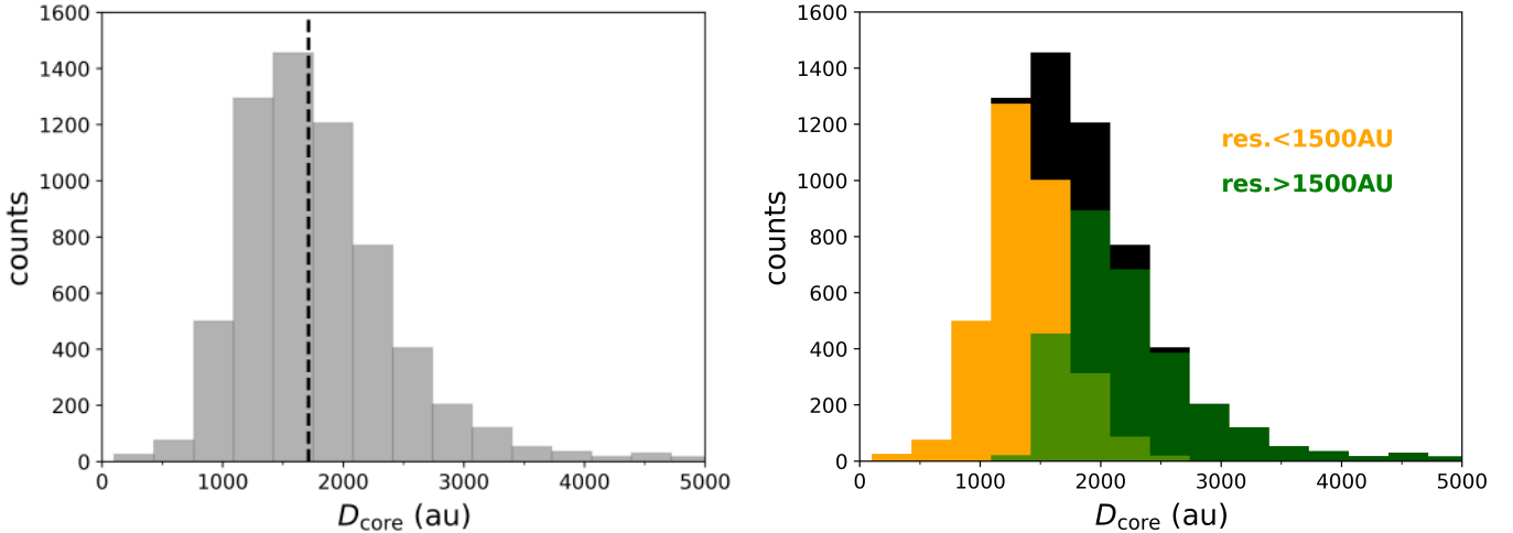
Fig. 14. Distribution of the cores’ estimated physical sizes (i.e., diameters). Left panel: overall distribution of core sizes. The vertical dashed black line marks the median value of the distribution (1700 au). For better visualization purposes, the few outliers above 5000 au ( \sim 2\% ) are not shown. Right panel: same distribution of left panel (black), but overlotted with the core size distributions resulting from better resolved fields (gold, below 1500 au) and less resolved ones (dark green, above 1500 au). The two histograms overlap in the lighter green area.
