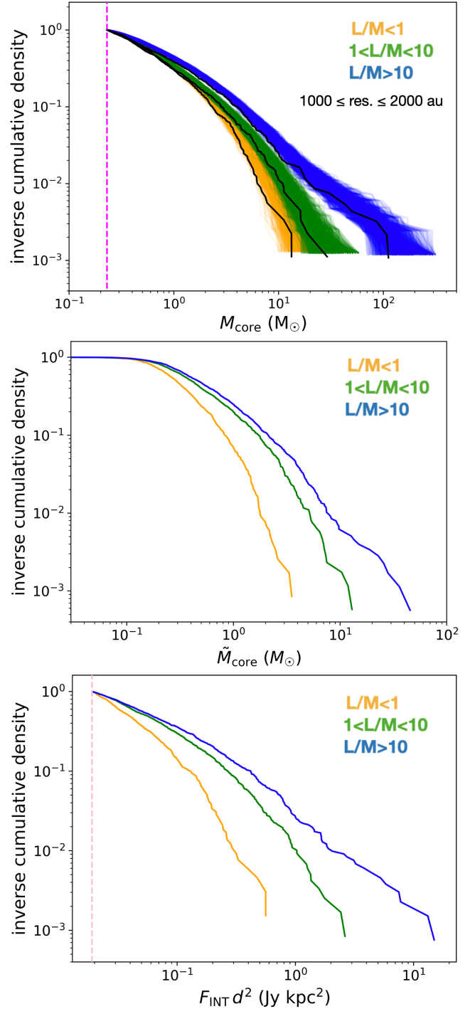
Fig. E.1. Analysis conducted to test the result of Fig. 18. Top panel: Same as Fig. 18, but for a subsample of cores selected based on the spatial resolution of the corresponding continuum map (within 1000 – 2000 au). Middle panel: CMF for the three evolutionary groups with core masses obtained using the temperature model from Sadaghiani et al. (2020) (see text for explanation). Bottom panel: Distribution of the F_{\text{INT}} d^2 quantity for the three evolutionary groups, computed to obtain an analog of the CMF but without the influence of the core temperature assumption. The vertical dashed pink line marks the minimum threshold we imposed for the plotted quantity, calculated by converting our mass completeness limit.
