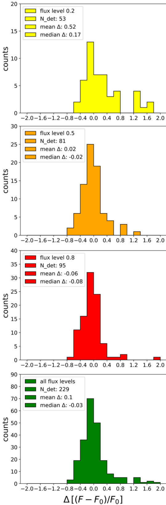
Fig. A.2. Same as panel b ) of Fig. A.1, but for the source extraction tests performed with the hyper code.
