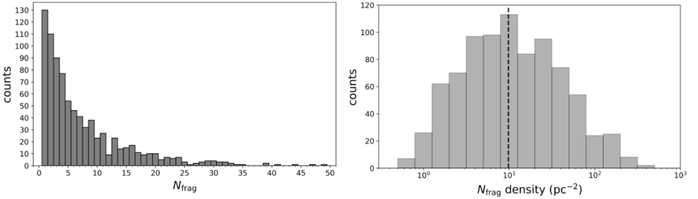
Fig. 8. Fragmentation statistics deduced from the compact source catalog (Table 3). Left panel: overall distribution of the number of cores detected in each clump; detailed statistics are reported in Table 4. Right panel: overall distribution of the derived spatial density of the cores in each clump, computed within the entire FOV. The vertical dashed black line marks the median value of \sim 10 \text{ pc}^{-2} . In both panels, only clumps revealing at least 1 detection are included.
