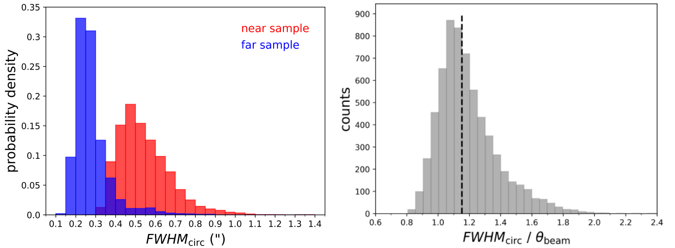
Fig. 12. Angular sizes of the extracted sources. Left panel: probability density distribution of the circularized FWHM of the sources. Red and blue bars include sources detected within the near sample and the far sample targets, respectively (see Sect. 2). Right panel: distribution of the ratio between the estimated angular size of the source and the map beam size (both in circularized form), providing a resolution-independent estimate of the source sizes. The vertical dashed black line marks the median value of 1.15 for the ratio.
