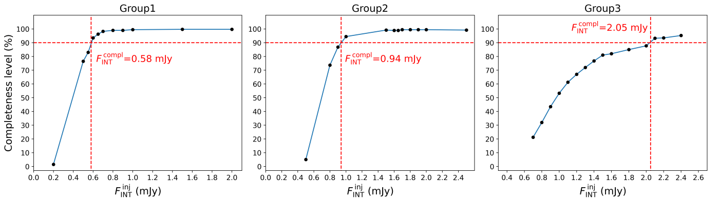
Fig. 7. Completeness levels (i.e., percentage of detection) as a function of the “true” integrated flux of the synthetic sources injected into the maps ( F_{\text{INT}}^{\text{inj}} ) for the three different groups of targets selected based on their rms noise, as introduced in Sect. 2.3: Group 1 (left panel), 2 (middle panel), and 3 (right panel), respectively. The two dashed red lines in each panel identify the estimated completeness flux, F_{\text{INT}}^{\text{compl}} , which is reported in red.
