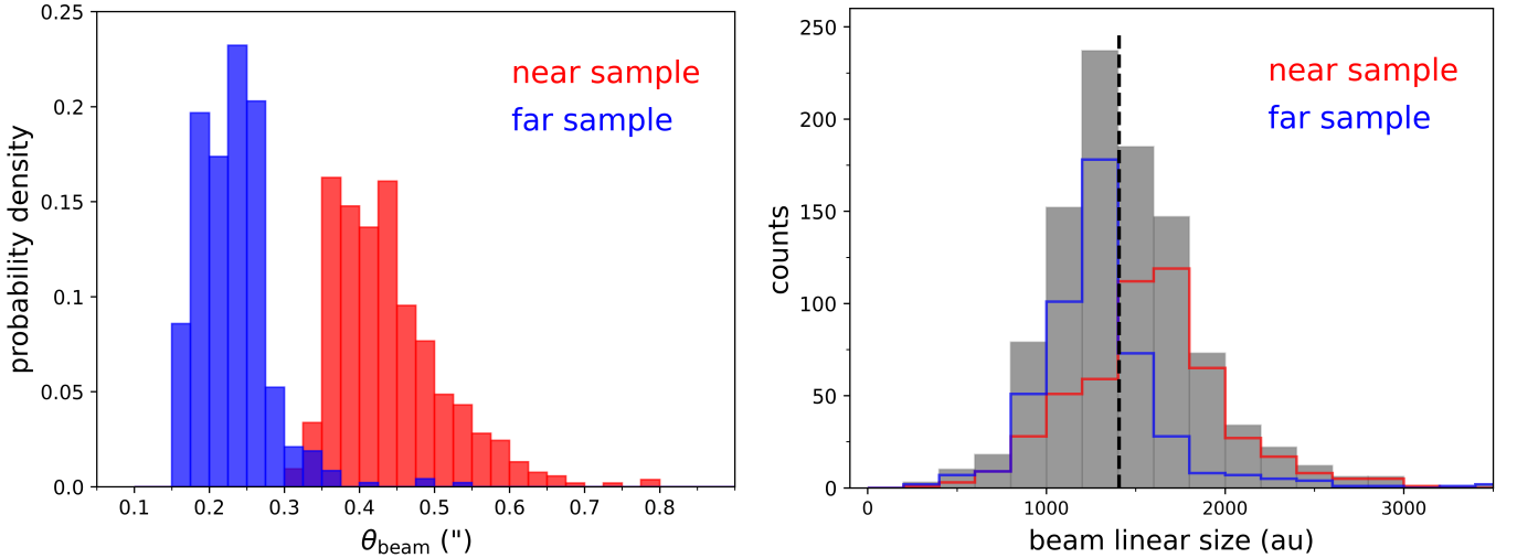
Fig. 1. Beam properties of the ALMAGAL continuum maps. Left panel: probability density distribution of the circularized angular sizes of the map beam, separately for near (red) and far (blue) observational samples, respectively (see Sánchez-Monge et al. 2025 for more details). Right panel: distribution of the corresponding linear sizes (i.e., achieved spatial resolution). The grey histogram represents the overall distribution, with the vertical dashed black line marking its median value (1400 au). Near and far subsamples are overlotted with the same color coding of the left panel. It can be noted that, due to the distance variation across our sample, the bimodal distribution in the left panel converts into a fairly uniform beam linear size overall distribution (see text for details).
