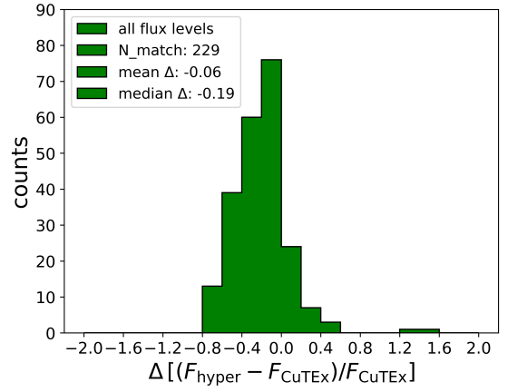
Fig. A.3. Histogram of the relative discrepancies (referred to as \Delta ) between the integrated fluxes measured by hyper and CuTEEx , for the matched synthetic sources combining all flux levels.
