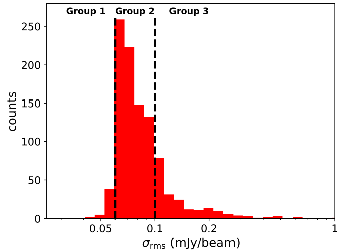
Fig. 3. Distribution of the map rms noise level \sigma_{\text{rms}} across the ALMAGAL maps sample (see Sánchez-Monge et al. 2025 for more details). The vertical dashed lines mark the subdivision into the three reported groups of fields that are employed in Sect. 3.3.
