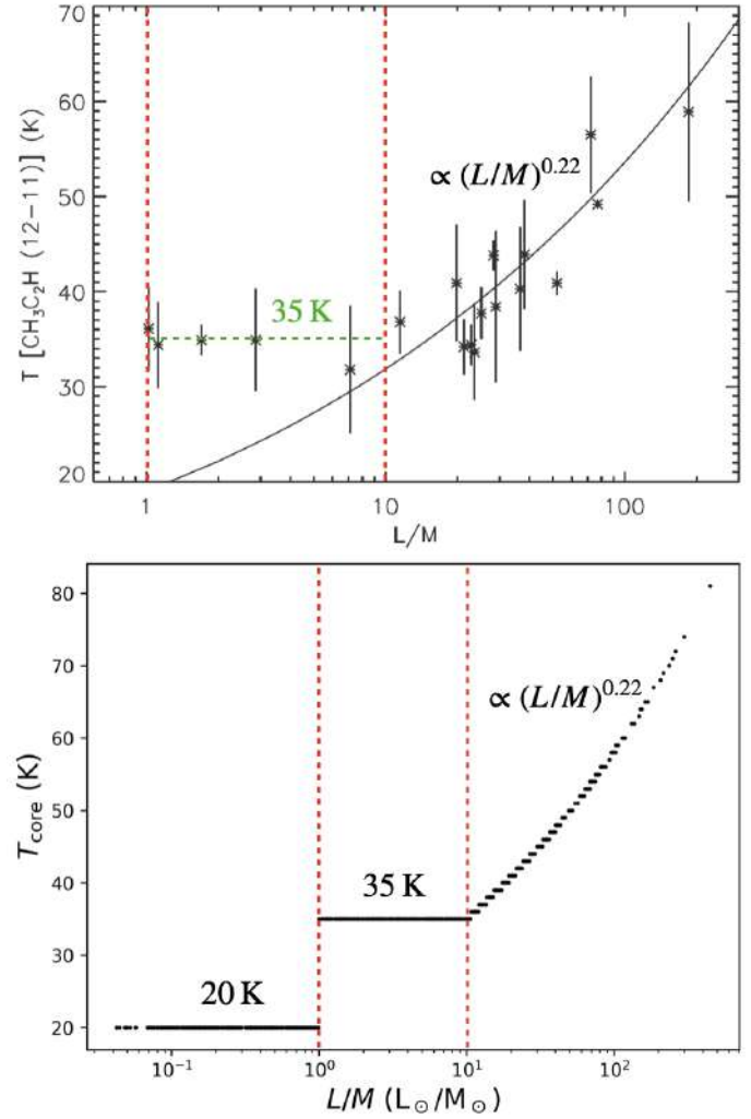
Fig. C.1. Details of the temperature model adopted for the cores. Top panel: Calibration of the clump L/M with the rotational temperature of \text{CH}_3\text{C}_2\text{H} , edited from Molinari et al. (2016a). The vertical dashed red lines mark different ranges of L/M as done in our work. The horizontal dashed green line mark the 35 K temperature value fitting the point within the 1 - 10 L_\odot/M_\odot range, which has been adopted in this work for the correspondent evolutionary group. The full black line represents the power law fitting the points at L/M > 10 L_\odot/M_\odot (see Molinari et al. 2016a), also adopted in this work. Bottom panel: Overall distribution of the assumed core temperatures as a function of the clump L/M , resulting from the model used in this work. The vertical dashed red lines serve as in the top panel.
