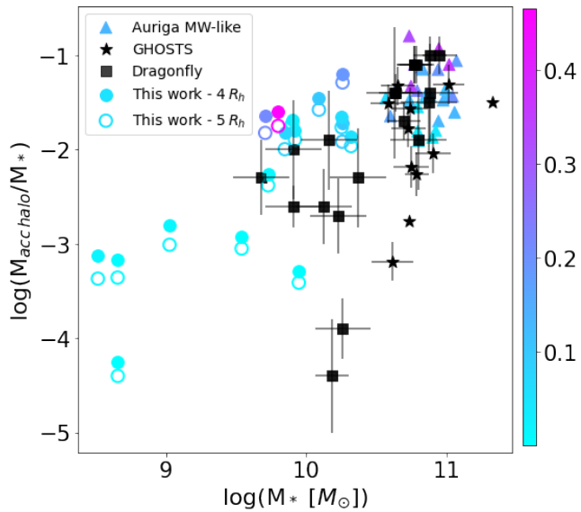
Fig. 6. Accreted stellar halo mass fraction as a function of the galaxies' total stellar mass. Filled circles represent computed mass fraction considering 4 R_h as the inner limit of the stellar halos, while empty circles consider this limit as 5 R_h . the Auriga MW-like galaxies are also shown, represented with triangles (Monachesi et al. 2019). All simulated galaxies are colour-coded with their accreted mass fraction. Observed galaxies taken from the GHOSTS (Harmsen et al. 2017; Gozman et al. 2023) and Dragonfly (Gilhuly et al. 2022) surveys are symbolised with stars and squares, respectively. The stellar halo fraction of the Dragonfly sample considered in this plot is the one computed outside 5 R_h of each galaxy.
