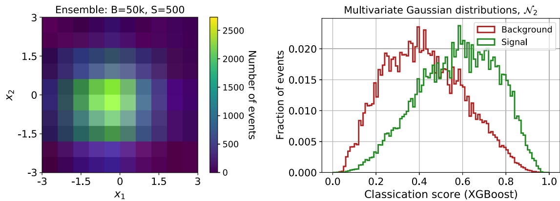
Fig. 2 Left panel: histogram of an hypothetical experiment with B = 50\text{k} and S = 500 events divided into 10 \times 10 bins. Signal and background distributions can be seen in Fig. 1. Right panel: classification score, o(x) , for a binary classifier using the XGBoost algorithm
