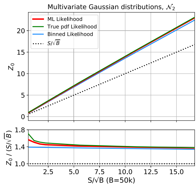
Fig. 3 Discovery significance calculated with various methods for the example in Fig. 2 for fixed background, \langle B \rangle = 50\text{k} , and different signal strengths \langle S \rangle . Red lines show the results implementing the ML Likelihood method with XGBoost used to estimate the probability density for single events and green lines when using the true multivariate distributions. The black dotted line represents the result of the usual counting method, S/\sqrt{B} , in the entire range of interest (only one bin), and the light blue curve the result of a binned counting experiment
