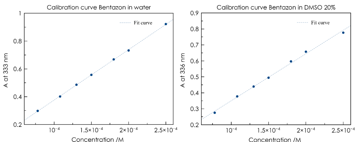
Figure SI-1. Calibration curve of Bentazon in water and DMSO/water 20%. The fitting linearization resulted in y = 3628,2x + 0,0134 R^2 = 0,9998 and y = 2948,7x + 0,0556 R^2 = 0,9963 respectively. The second calibration curve was used to assess indirectly the bentazon charge load from the supernatant from adsorption procedures. The results showed minimal discrepancy with the Elemental Analysis that were thus selected as most accurate method.
