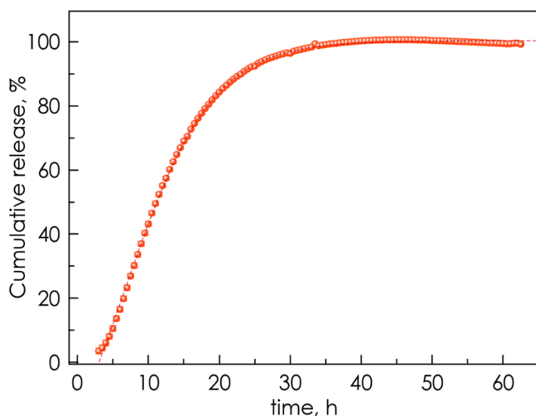
Figure SI-5. Btz release in aqueous media at pH of 4,5 in acetate buffered solution, experimental results are average of triplicates and errors are reported in the graph. Dotted line represents the best fit to the experimental data. Release constant resulted in k=0,20 \text{ h}^{-1} for the release in acetate buffer. This result show a 2 times higher kinetics than in neutral Tris-HCl buffered media.
