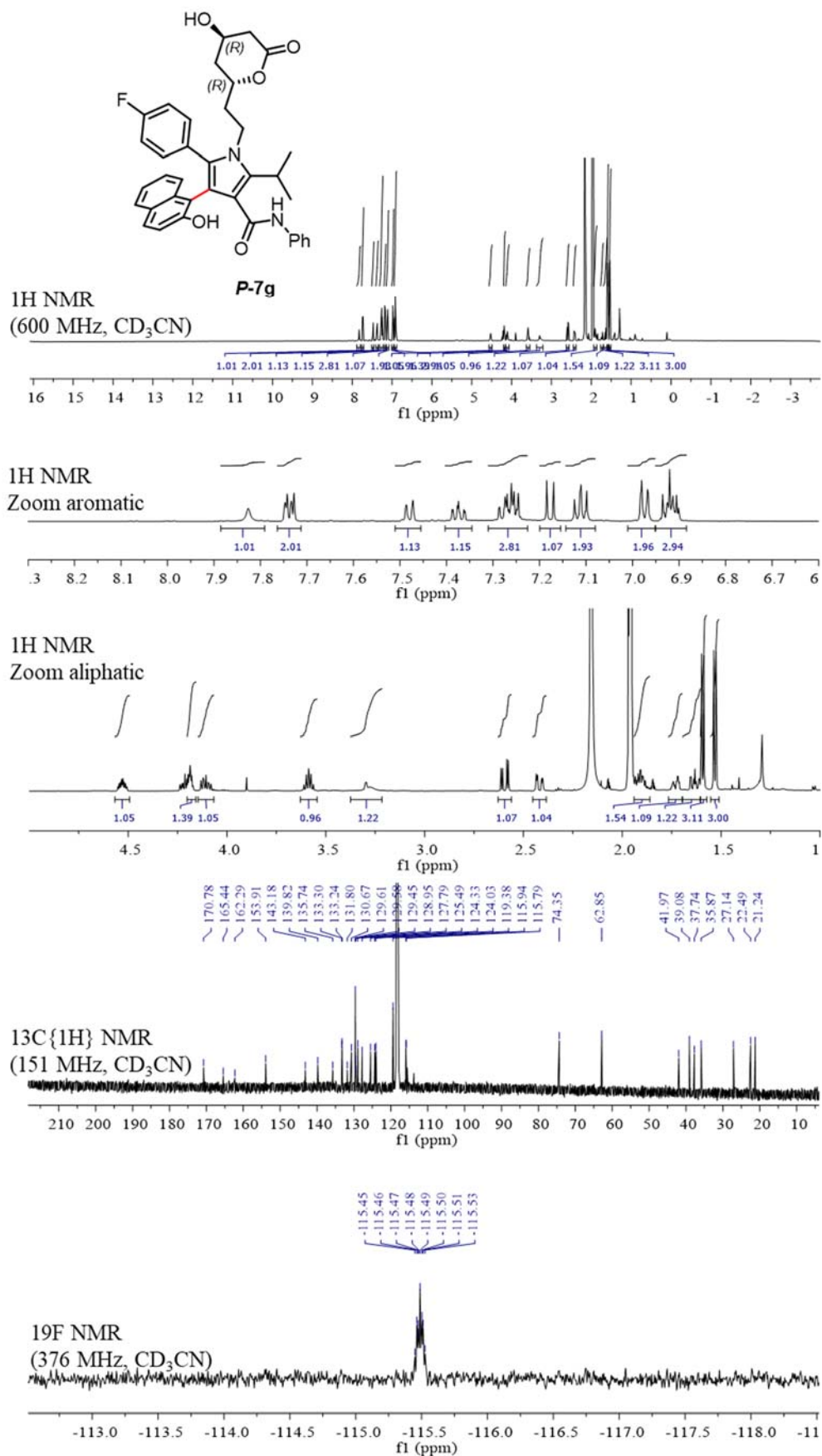
Figure S60. NMR spectra of P-7g in CD 3 CN.
