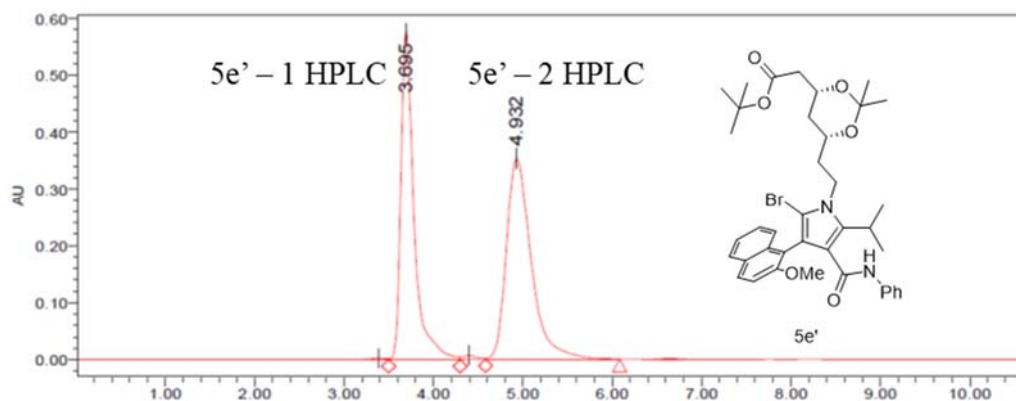
Figure S9. CSP-HPLC chromatogram of 5e' . Separation in AD-H column, 80:20 Hex/IPA, 20 mL/min, first eluted = 3.7 min, second eluted = 4.9 min).
