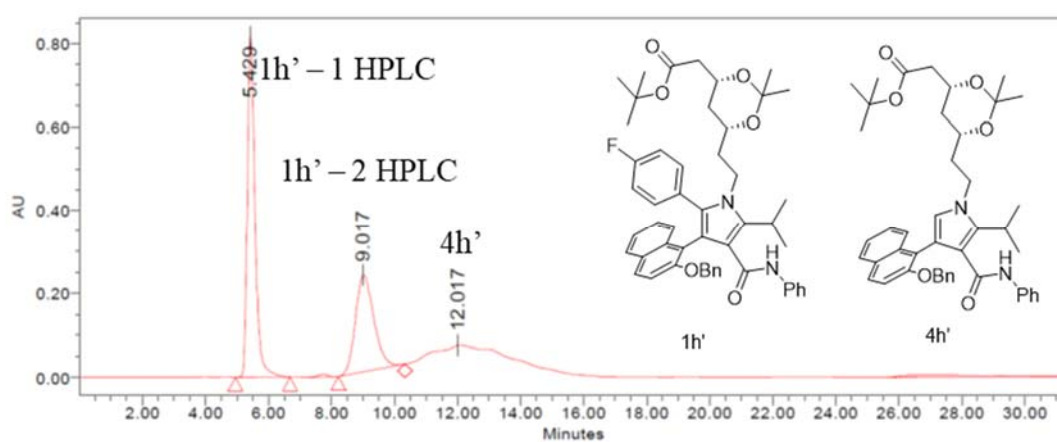
Figure S12. CSP-HPLC chromatogram of 1h' and 4h' . Separation in AD-H column, 90:10 Hex/IPA, 20 mL/min, first eluted = 5.4 min, second eluted = 9.0 min, 4e' eluted = 12.0 min).
