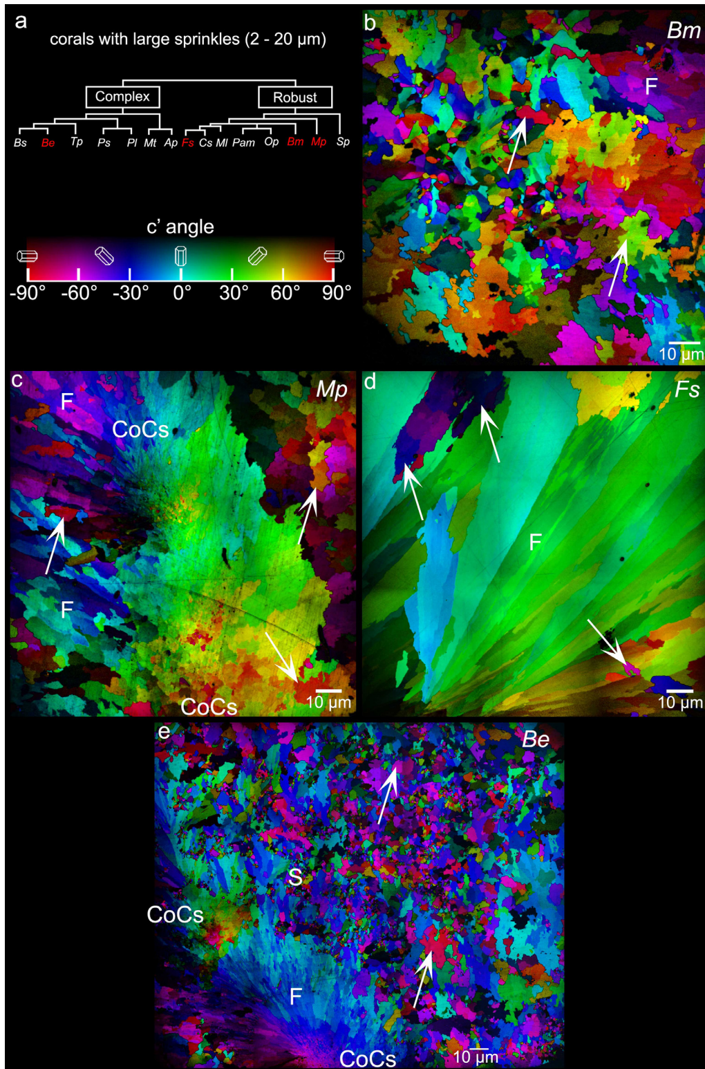
Fig. 4. PIC maps of the 4 coral species that exhibit large (2–20 \mu\text{m} ) sprinkles across their skeletons. These are Blastomussa merleti ( Bm ), Madracis pharensis ( Mp ), Favia sp. ( Fs ), and Balanophyllia europaea ( Be ). Arrows indicate a few large sprinkles, but many more are visible. Large sprinkles are distinct from fibers (F) not by size but by crystal orientations: they form > 35^\circ angles with their neighboring crystals, whereas fiber crystals only form small angles ( < 35^\circ ) with respect to adjacent fibers in the same bundle. Nanoparticulate crystals (between pairs of CoCs labels) are visible in the CoCs of Mp and Be . Nanocrystals in the CoCs are not randomly oriented, but rather oriented similarly to their neighboring crystals. CoCs, therefore, cannot be sprinkles. (For interpretation of the references to color in this figure, the reader is referred to the web version of this article.)
