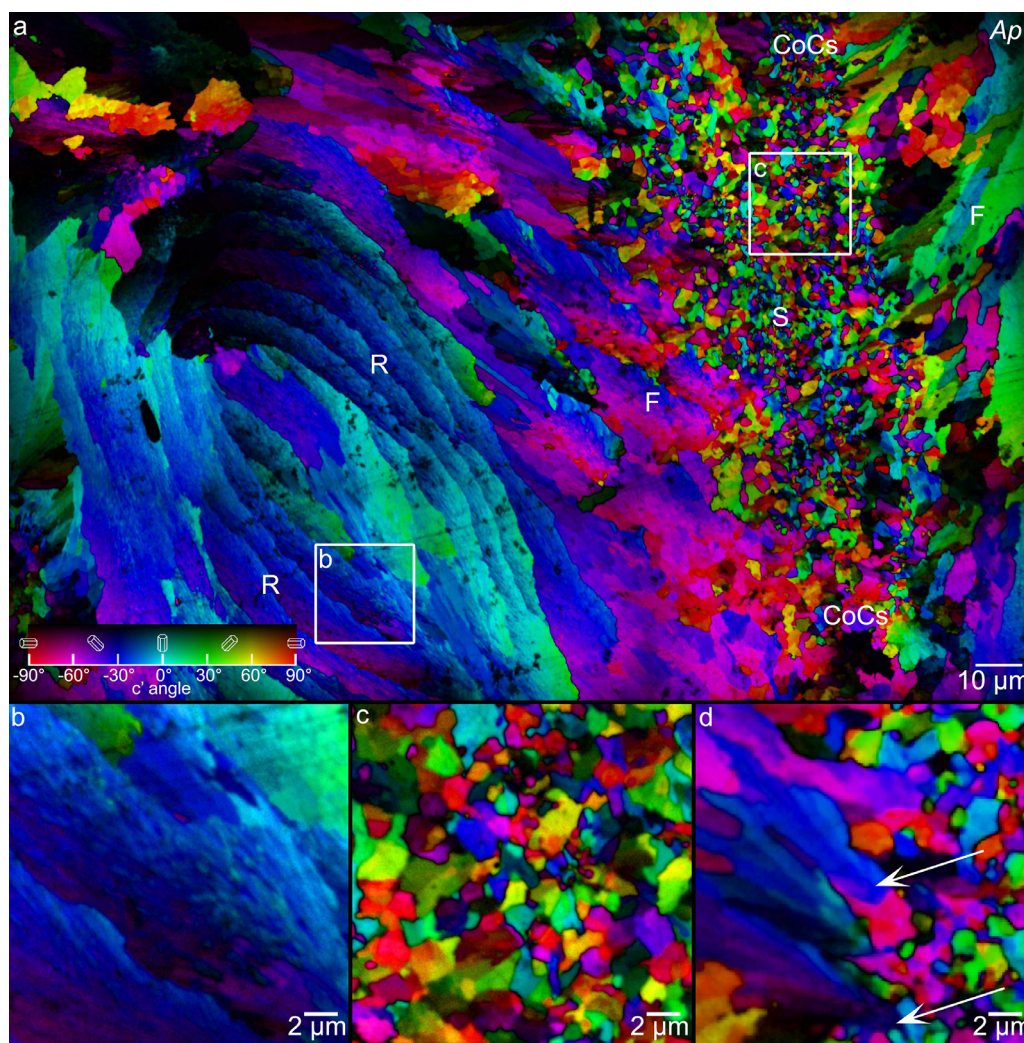
Fig. 6. a: PIC map of Acropora pharaonis (Ap) coral skeleton, showing sprinkles (S) concentrated at the CoCs (between pairs of CoC labels), spherulitic crystal fibers (F) fanning out from the CoCs, and concentric rings (R), which consist of finer spherulitic fiber crystals. Boxes b, c indicate the areas magnified in panels b, c. b: Magnified concentric rings, showing that these are made of nearly co-oriented acicular crystals. c: Magnified sprinkles from CoCs. d: Sprinkles at the boundary of CoCs and fiber crystals, magnified from the box area in Fig. 3d. Arrows indicate two blue sprinkles that expand radially into -30^\circ oriented fibers. Red and green sprinkles do not grow as they run into other crystals. In panels a and d pixels are 60 nm, in b and c they are 20 nm. (For interpretation of the references to color in this figure legend, the reader is referred to the web version of this article.)
