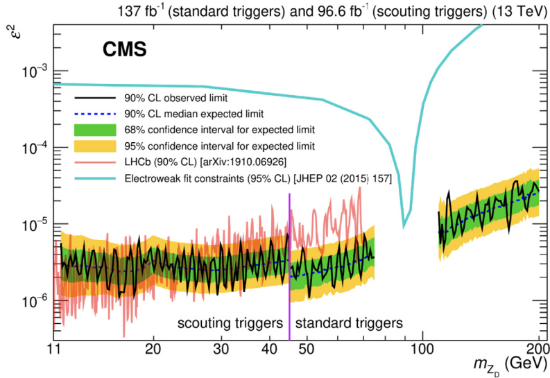
Fig. 18. Expected and observed upper limits at 90% CL on the square of the kinetic mixing coefficient ( \epsilon^2 ) as a function of dark photon mass. Results obtained with scouting triggers are displayed to the left of the vertical purple line, while those obtained with standard triggers are shown to the right. Limits at 90% CL obtained from the search performed by the LHCb Collaboration [90] are shown in red, and constraints at 95% CL from the measurements of electroweak observables are shown in light blue [91]. Source: Figure taken from Ref. [68].
