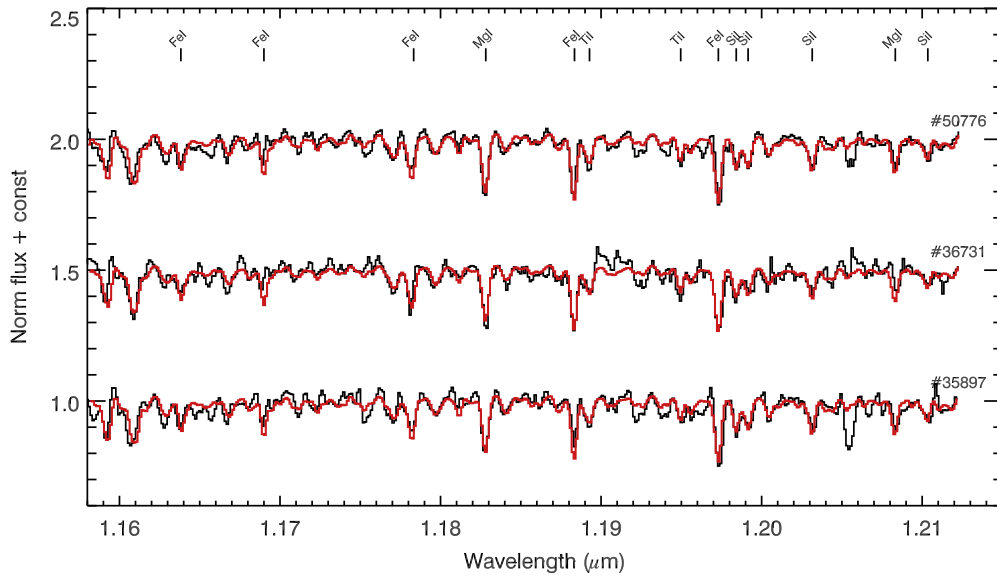
Figure 3. Spectra of the targeted SSCs in the J -band window, along with the best-fit spectra (red lines).
