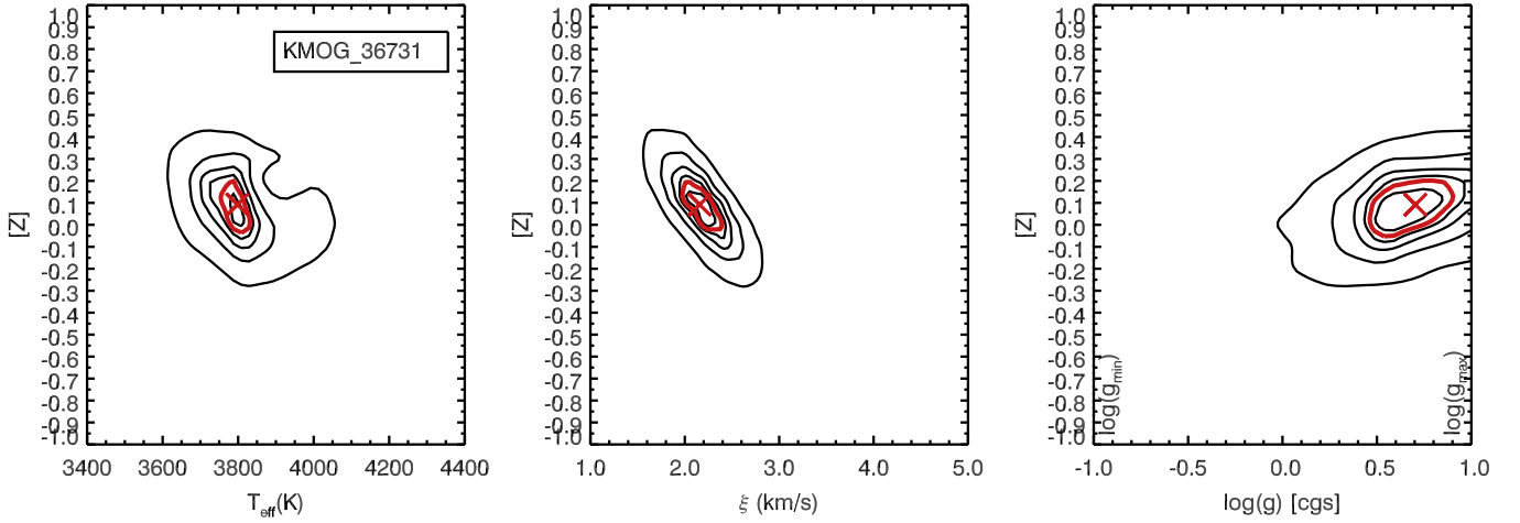
Figure 4. Planes through the model grid showing the degeneracy between the parameters for the analyzed SSCs. The black contours show contours of equal \chi^2 , and are drawn at levels of \chi_{\min}^2 + (1, 2, 3, 5, 10) . The red contour is drawn at \chi^2 = \chi_{\min}^2 + 3 , which indicates our 1\sigma uncertainty. The x-axis limits on the right-hand plot are the minimum and maximum possible values of \log g allowed by the object’s temperature and luminosity.
