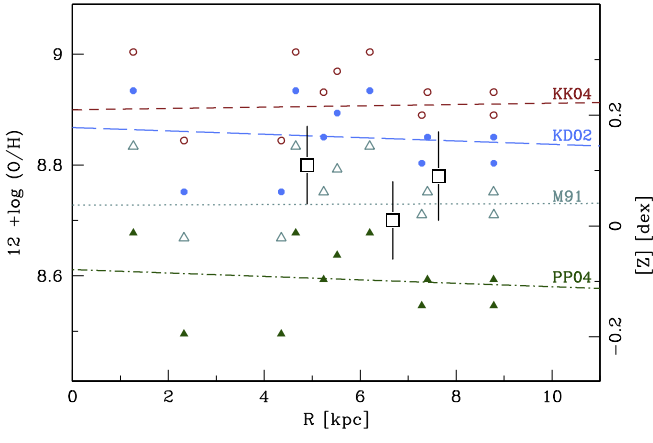
Figure 5. Direct metallicities from the SSC analysis (large squares) are shown together with the H II region metal abundances by Bastian et al. (2009) as a function of galactocentric radius. Small symbols are the abundances obtained from different strong-line calibrations to the data of Bastian et al. (2009): Kobulnicky & Kewley (2004, KK04 ; red empty circles, adopted by Bastian et al. 2009), Kewley & Dopita (2002, KD02 ; blue filled circles), McGaugh (1991, M91 ; teal empty triangles), and Pettini & Pagel (2004, PP04 ; green filled triangles).
