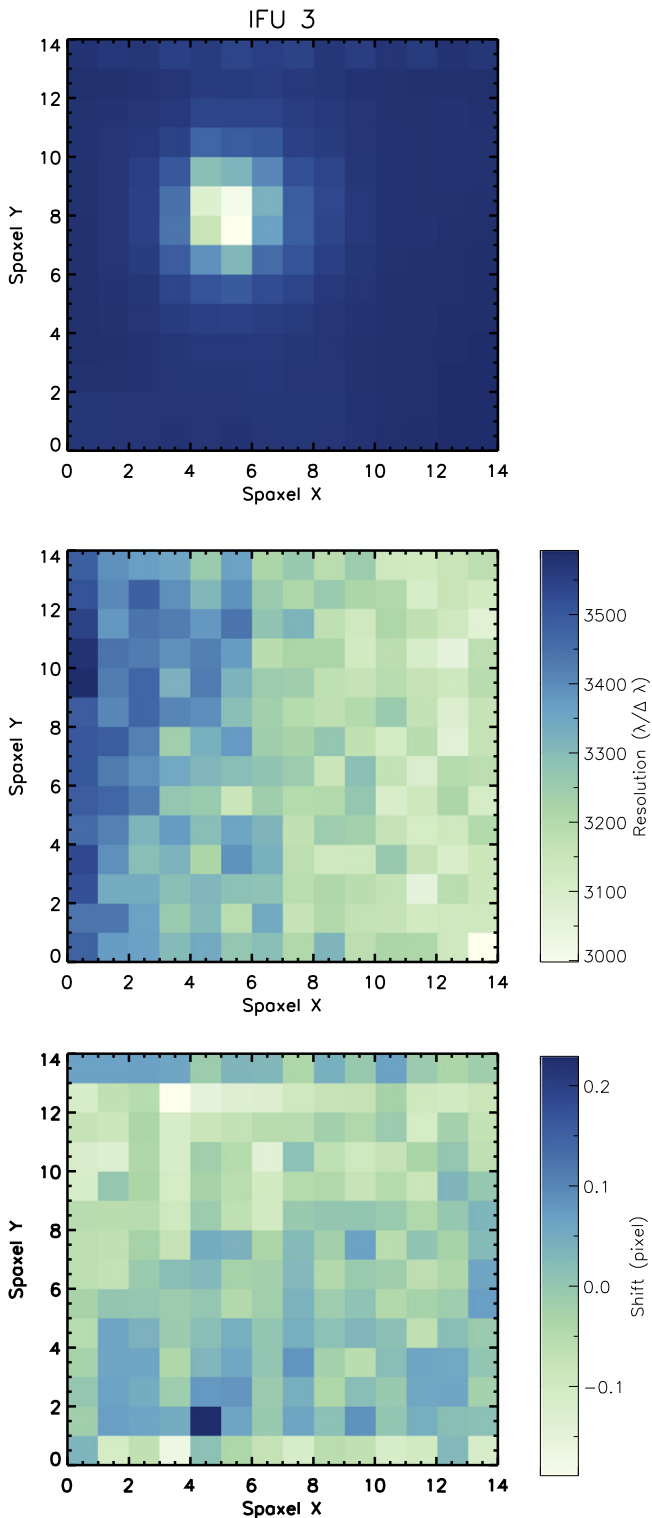
Figure 2. Variation of spectral resolution and wavelength calibration across the spatial pixels of a typical KMOS IFU measured from night sky lines. The top panel presents the reconstructed image obtained in a 300 s exposure. The middle and bottom panels show the variation of spectral resolution and the wavelength shifts (in pixels) across the spaxels, respectively.
