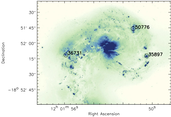
Figure 1. Targeted SSCs are overlaid on a HST -ACS F814W image of NGC 4038 retrieved from the Hubble Legacy Archive ( http://hla.stsci.edu/hlaview.html ).
