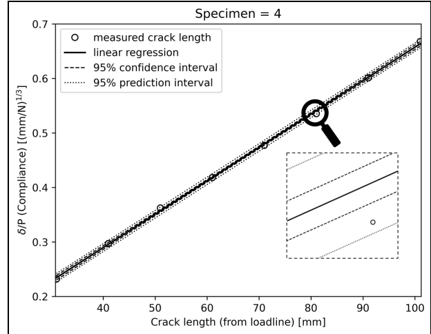
Figure 5. Compliance calibration.
