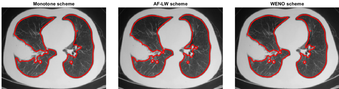
Figure 19: Test 6a with Datum 2. From left to right: Plots of the final front using the monotone scheme ( N_i = 413 ), tol = 0.00001 , the AF-LW scheme ( N_i = 589 ) with tol = 0.00001 , and the WENO scheme ( N_i = 458 ) with tol = 0.000012 , all using L^1 norm, \mu = 4 , K_{reg} = 5 , and velocity \tilde{c} .
