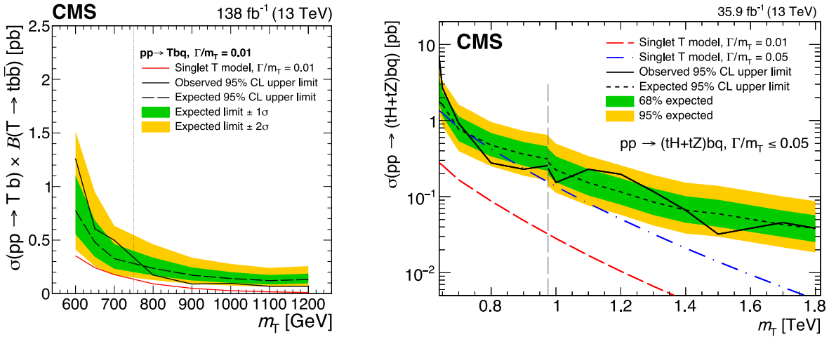
Fig. 23. Observed and median expected upper limits at 95% CL on the cross sections for single T quark production associated with a b quark, for the sum of t\bar{H}bq and tZbq channels, as a function of the assumed values of the T quark mass. The inner (green) band and the outer (yellow) band indicate the regions containing 68 and 95%, respectively, of the distribution of limits expected under the background-only hypothesis. The left figure corresponds to the analysis strategy described in Ref. [148], based on the five-jet invariant mass reconstruction of the T . The figure on the right corresponds to the analysis strategy in Ref. [145], which employs different reconstruction algorithms for the low- and high-mass searches. The vertical dashed lines represent the crossover point in sensitivity for the low-mass and high-mass selections. Source: Figures adapted from Refs. [145,148].
