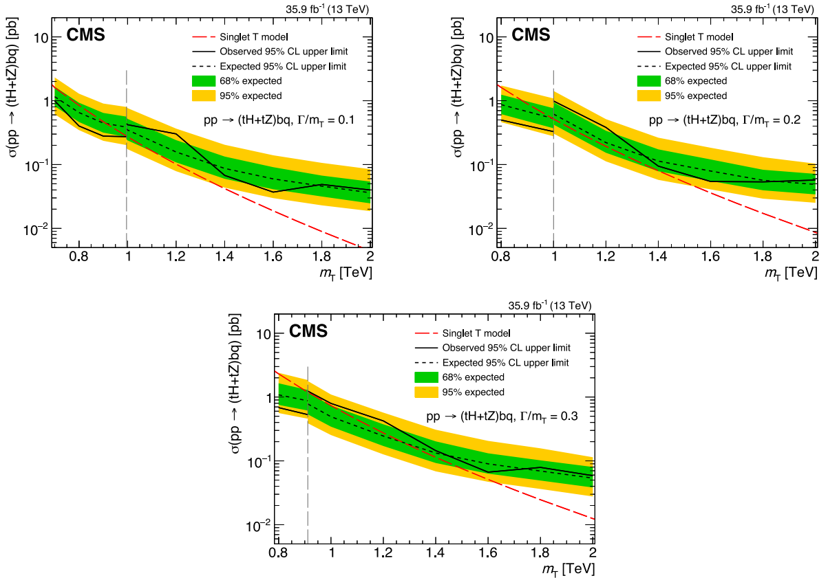
Fig. 24. Observed and median expected upper limits at 95% CL on the cross sections for single T quark production associated with a b quark, for the sum of t\bar{H}bq and tZbq channels, as a function of the assumed values of the T quark mass. The inner (green) band and the outer (yellow) band indicate the regions containing 68 and 95%, respectively, of the distribution of limits expected under the background-only hypothesis. The results are given for relative widths of \Gamma/m_T = 10 (upper left), 20 (upper right), and 30% (lower). The vertical dashed lines represent the crossover point in sensitivity for the low-mass and high-mass selections. Source: Figures adapted from Ref. [145].
