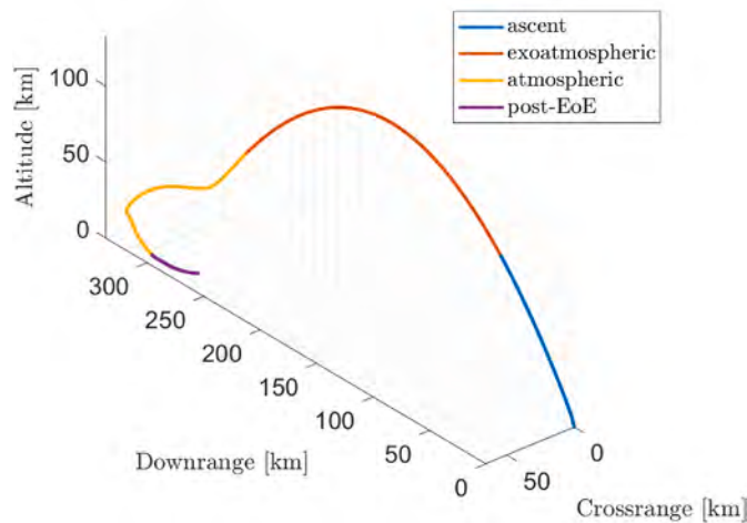
Fig. 11. ReFEx mission phases and events.
