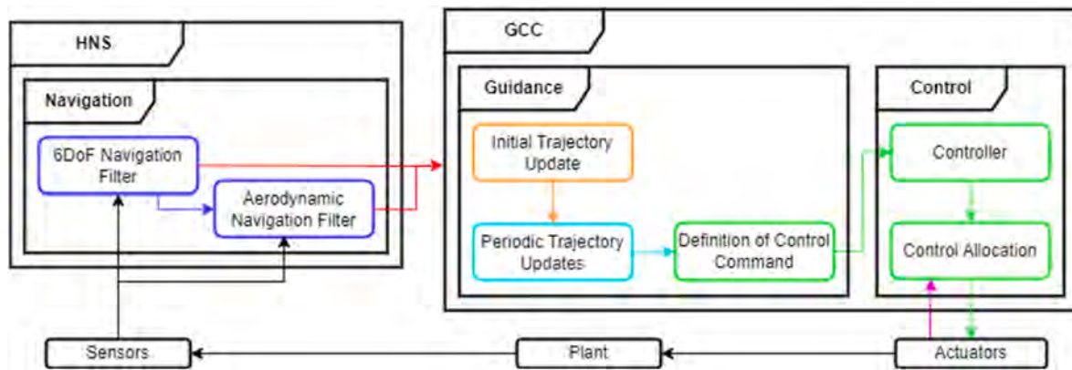
Fig. 13. ReFEx high-level GNC logic.
