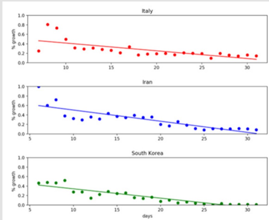
Figure 1: Linear model of the growth rate of the coronavirus.
