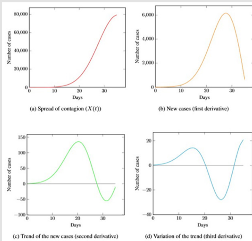
Figure 2: Possible model of Italy. The main aspect to be noted is the trend disregard specific numbers, which could contain significant errors due to the mathematical operations performed on them. The data is publicly available at [23, 8].
