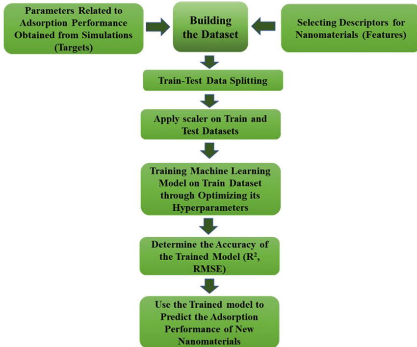
Figure 5: Flow chart representing the steps involved in training machine learning models.
