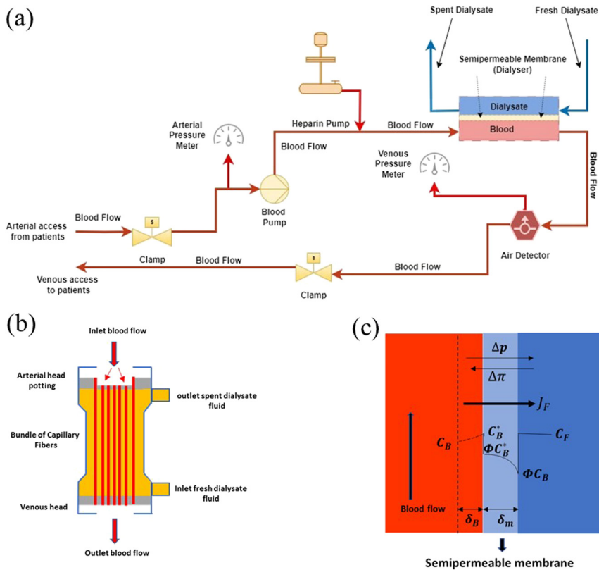
Figure 1: Conventional HD equipments. (a) The diagram of conventional HD, (b) the schematic of dialyser having hollow fibres, (c) convective solute transport across a semipermeable membrane in a hemodiafiltration process. Symbols are defined in the text.
