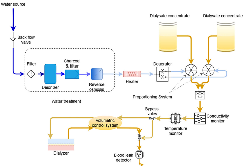
Figure 2: Conventional dialysate circuit.
