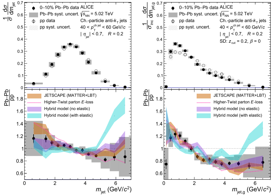
Fig. 1. ALICE measurements of ungroomed m_{\text{jet}} (left) and groomed m_{\text{jet,g}} (right) using R = 0.2 charged-particle jets with 40 < p_T^{\text{ch,jet}} < 60 GeV/c in pp and Pb-Pb collisions at \sqrt{s_{\text{NN}}} = 5.02 TeV compared to models. The bottom panel shows the ratio of Pb-Pb distributions to pp, which quantifies the substructure modifications from quenching.
