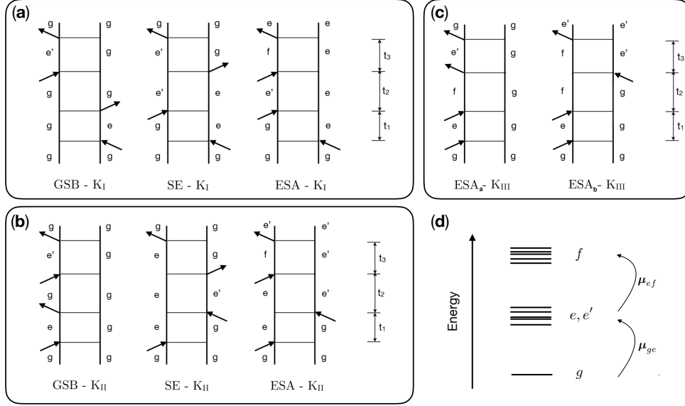
Figure 2: Ladder diagrams for the signal generated in the direction \mathbf{K}_I (a), \mathbf{K}_{II} (b) and \mathbf{K}_{III} (c); GSB: ground-state bleaching; SE: excited-state emission; ESA: excited-state absorption. (d) Energy level diagram and allowed transitions between the states in the various manifolds.
