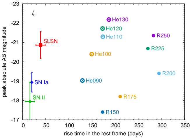
Fig. 2. Rise times and peak absolute magnitudes of the PISN and SLSN models in the rest frame in the I_E band. The PISN models (R250, R225, R200, R175, R150, He130, He120, He110, He100, and He090) are from Kasen et al. (2011) and the SLSN template is from Moriya et al. (2022). We also show rise times and peak absolute magnitudes of the SN Ia template from Hsiao et al. (2007) and the SN II Nugent template for comparison (see Sect. 5 for details). The error bars in the SLSN, SN Ia, and SN II templates show a typical dispersion (e.g., Richardson et al. 2014; Miller et al. 2020; González-Gaitán et al. 2015).
