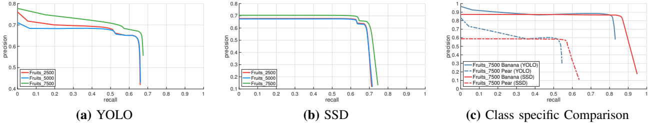
Fig. 7: Precision/Recall curves for the two type of detector trained on different subsets of the Fruits dataset. (a) and (b) report the results for YOLO and SSD respectively; (c) instead displays a comparison between SSD and YOLO over the best class ( Banana ) and the worst class ( Pear ) of the Fruits dataset.
