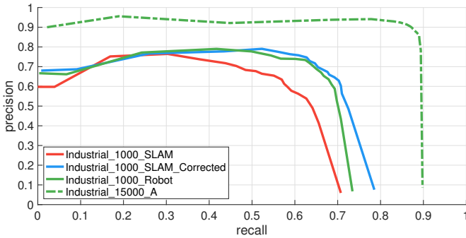
Fig. 8: Precision/Recall curves for the YOLO detector trained on a subset of the Industrial dataset where the camera is also tracked with the Orb-Slam-v2 algorithm[23].
