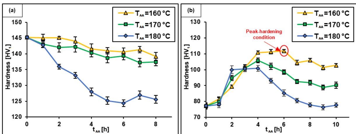
Fig. 11. Aging curves related to the conditions: (a) AB, (b) SHTR LPBF AISi10Mg alloy at 160 °C, 170 °C, 180 °C.
