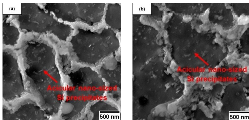
Fig. 8. LPBF AlSi10Mg alloy microstructures: (a) AB; (b) T5: T_{AA}=160\text{ °C} t_{AA}=4\text{ h} .
