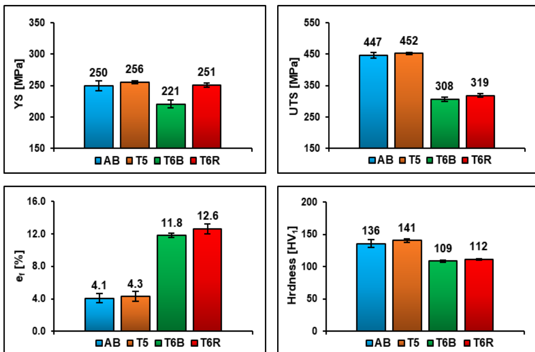
Fig. 12. Tensile properties and hardness of the LPBF AISi10Mg alloy related to the conditions: (i) AB, (ii) T5 (AA at 160 °C for 4 h), (iii) T6B (SHTB at 540 °C for 1 h and AA at 160 °C for 4 h) and (iv) T6R (SHTR at 510 °C for 10min and AA at 160 °C for 6 h).
