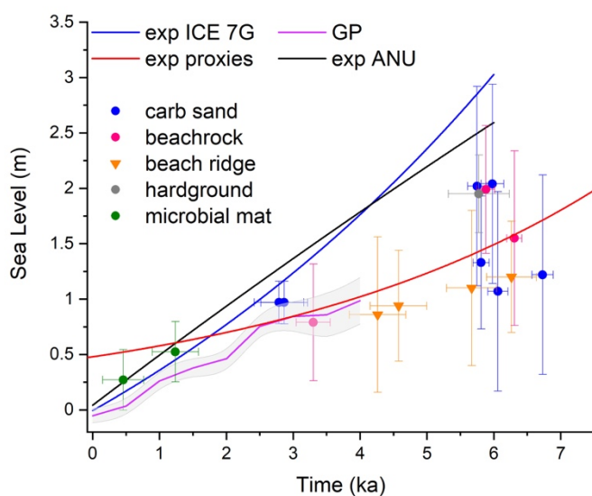
Fig. 6. The curves resulting from the exponential decay fit of ICE-7G (blue), ANU (black) and proxy data (red; data points representing transgression excluded). Gaussian Process (GP) model curve (purple) and proxy data are also plotted. For details of fits see Figs S2 and S3.
