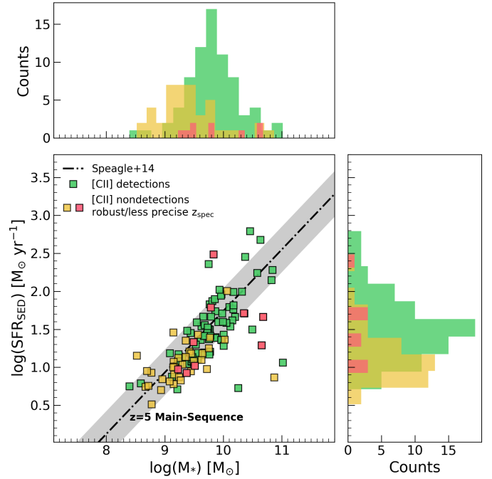
Fig. 1. SFRs vs stellar masses of the ALPINE [CII]-detected (green squares) and undetected (yellow squares) galaxies. Red symbols represent [CII] nondetections with less precise spectroscopic redshift (see Sect. 2.2). The main-sequence of star-forming galaxies by Speagle et al. (2014) is shown as the black dot-dashed line, with its \pm 0.3 dex width represented by the gray shaded region. Top and right panels report the distributions in stellar mass and SFR, respectively, for both the detections and nondetections.
