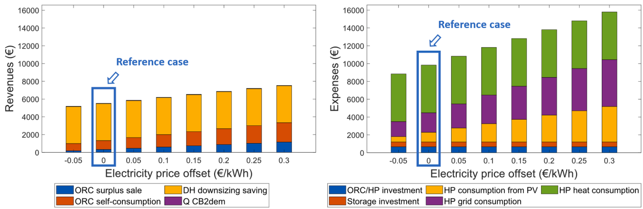
Fig. A10. Carnot battery annual revenues and expenses when varying the electricity price of an offset for the 2nd reference case.
