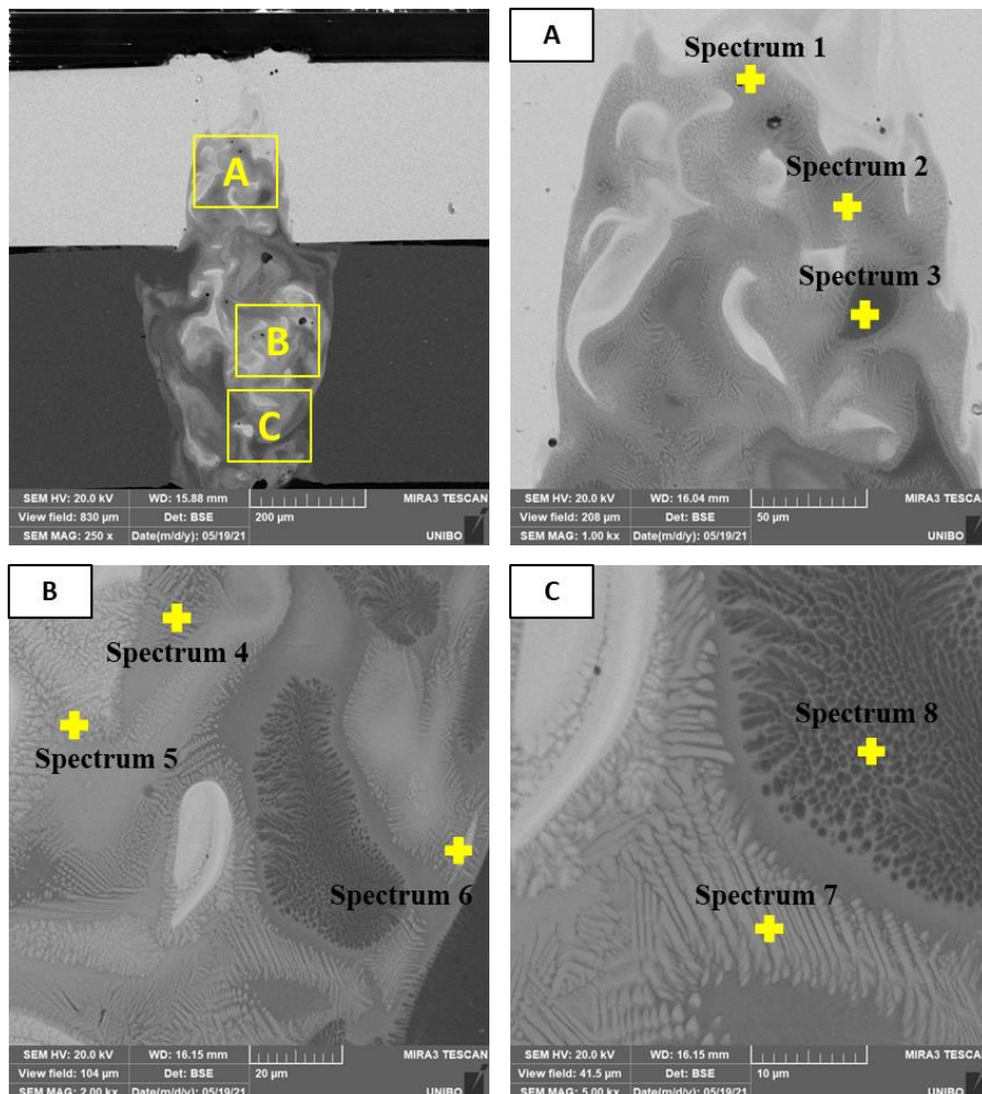
Fig. 9: SEM images of sample C3; Power = 1000 W, Welding Speed = 250 mm/s, Spot diameter = 68 μm
