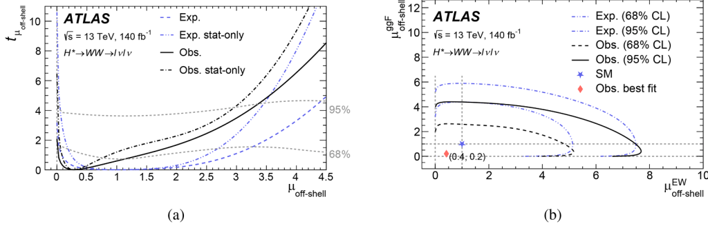
Fig. 3. (a) Values of the test statistic t_{\mu_{off-shell}} as a function of the off-shell Higgs boson signal strength, \mu_{off-shell} . The 68 % and 95 % CL are shown as gray dotted lines. (b) Contours of the values of the profile likelihood ratio t_{\mu_{off-shell}^{ggF}, \mu_{off-shell}^{EW}} as a function of \mu_{off-shell}^{ggF} and \mu_{off-shell}^{EW} . The SM predicted value and best-fit value are indicated by a star and a diamond, respectively. The observed (expected) results are shown in black (blue) for scenarios with and without systematics. For (a) the 68 % and 95 % CL are calculated using an explicit Neyman construction, whereas in (b) they are calculated via the asymptotic approximation. (For interpretation of the references to color in this figure legend, the reader is referred to the web version of this article.)
