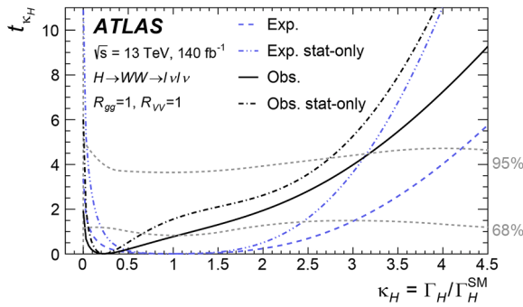
Fig. 4. Values of the test statistic t_{\kappa_H} as a function of \kappa_H = \Gamma_H / \Gamma_H^{SM} for the combined on-shell and off-shell result assuming R_{gg} = R_{VV} = 1 . The observed (expected) results are shown in black (blue) for scenarios with and without systematics. The 68 % and 95 % CL are shown as gray dotted lines. The 68 % and 95 % CL were calculated using an explicit Neyman construction. (For interpretation of the references to color in this figure legend, the reader is referred to the web version of this article.)
