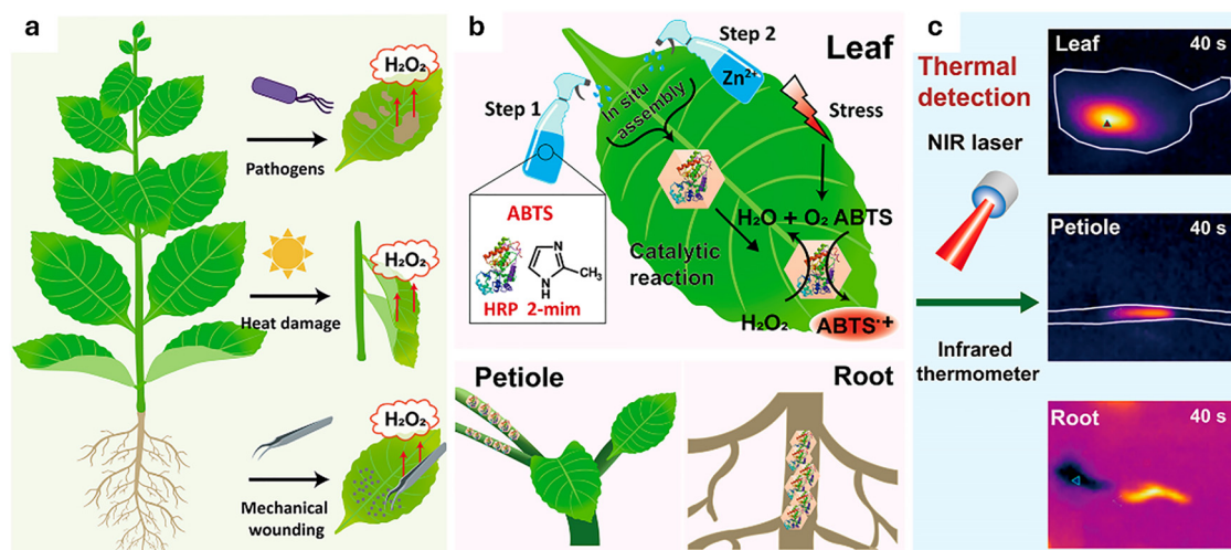
Fig. 37 (a) Schematic representation of the external factors that induce ROS, e.g., \text{H}_2\text{O}_2 , formation in plants. (b) The MOF nanosensor was used to detect \text{H}_2\text{O}_2 on plant leaves, stems, and roots. (c) \text{ABTS}^{\bullet+} generates thermal signals under a NIR laser that are detectable by a thermometer. Figure reproduced with permission from ref. 653.
