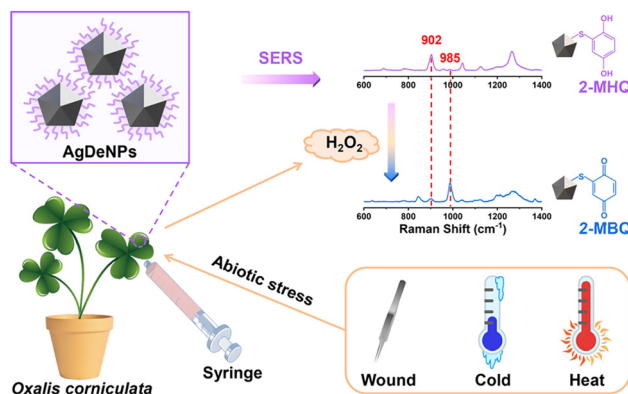
Fig. 44 Schematic illustration of the SERS-based detection of \text{H}_2\text{O}_2 by \text{AgDeNPs}@2\text{-MHQ} in Oxalis corniculata leaves subjected to abiotic stresses, such as heat and mechanical damage. Figure reproduced with permission from ref. 647.
