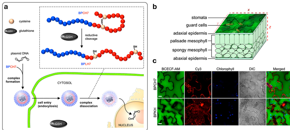
Fig. 77 (a) Schematic representation of the glutathione-reducible peptide (BPCH7) and the proposed mechanism for intracellular delivery and subsequent pDNA release. BPCH7 (KKLFKILKYLHHCGRGHTVHSHHHICIR) forms a stable complex with plasmid DNA in the extracellular environment. Once the complex is delivered into the plant cell via endocytosis, the reductive intracellular environment, primarily mediated by glutathione (GSH), triggers the cleavage of the intramolecular disulfide bond within the cyclic CH7 domain. This cleavage leads to the dissociation of the complex and the subsequent release of pDNA, allowing its expression in the cell nucleus. (b) Cartoon of a leaf indicating locations of the adaxial and abaxial epidermis as well as palisade and spongy mesophyll cells. (c) Confocal images taken from vacuolar compartmentation of BCECF-AM in wild-type A. thaliana leaf epidermal cells. Scale bars indicate 10 \mu\text{m} . Figure reproduced with permission from ref. 796.
