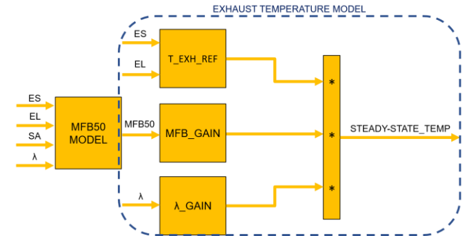
Figure 2. Block-layout of the exhaust gas temperature model. The reference temperature is multiplied by two factors that depend on MFB50 and lambda values respectively. The MFB50 model from [4] allows to calculate the combustion phase without the need for indicating signals.
