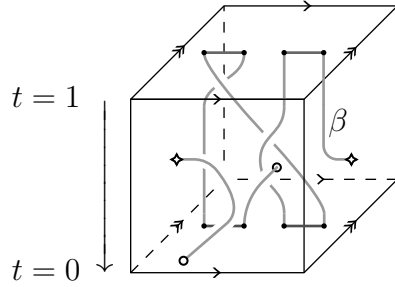
Figure 2: An example of a closure \widehat{\beta} with \beta \in B_{1,4} .
