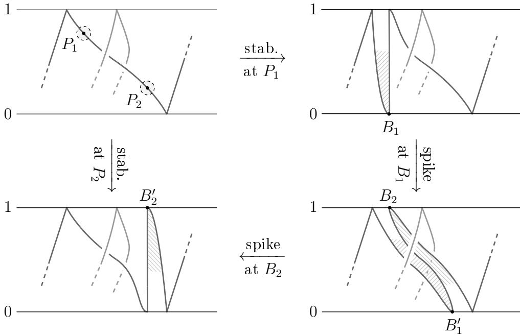
Figure 9: Normalizing the stabilization: always done at the bottom right of an even strand.
