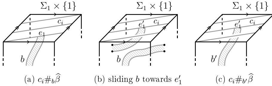
Figure 15: Normalizing the plat slide move.
