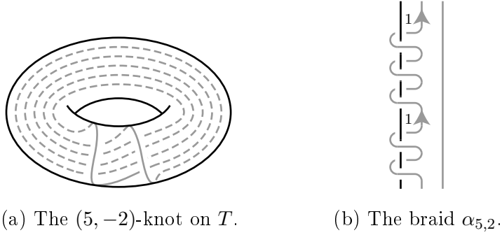
Figure 17: Braiding of the torus knot (5, -2) .
