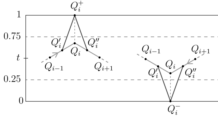
Figure 3: The braiding process.
