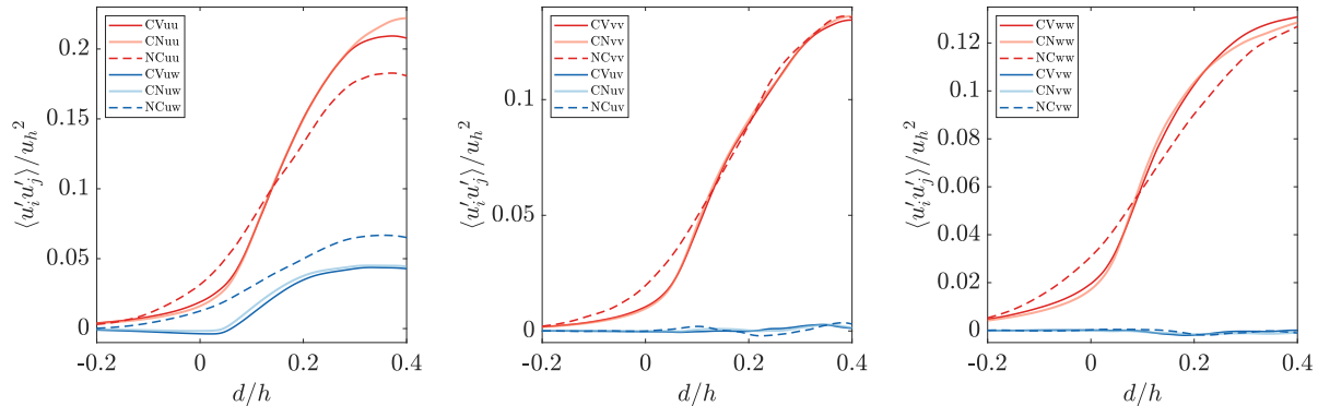
FIG. 7. Reynolds stresses \langle u'_i u'_j \rangle (see legend) normalised with u_h^2 as a function of distance d/h from the interface for separation vector r/h = 0.0 at time t = 140 . Positive d indicates the turbulent zone towards the centre of the jet. CV, CN and NC represent vertical conditional, normal conditional and non-conditional averaging, in dark, light and dashed lines, respectively.
