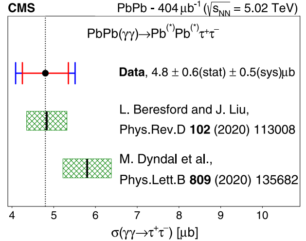
FIG. 3. The cross section, \sigma(\gamma\gamma \rightarrow \tau^+\tau^-) , measured in a fiducial phase space region at \sqrt{s_{NN}} = 5.02 TeV. The theoretical predictions [3,4] are computed with leading-order accuracy in QED and are represented by the vertical solid lines that can be compared with the vertical dotted line representing this measurement. The outer blue (inner red) error bars surrounding the data point indicate the total (statistical) uncertainties, whereas the green hatched bands correspond to the uncertainty in the theoretical predictions as described in the main text. The potential electromagnetic excitation of the outgoing Pb ions is denoted by (*).
