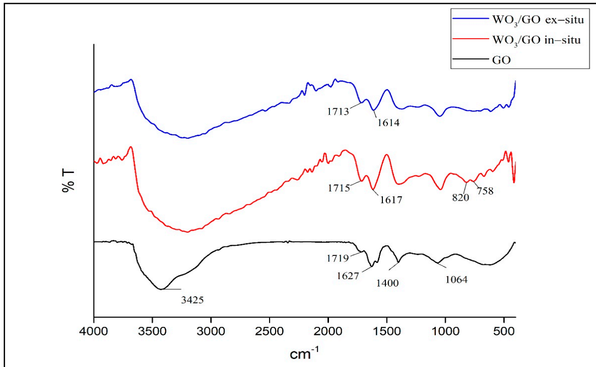
Figure 4. FTIR Spectra of GO and WO 3 /GO Composites.
