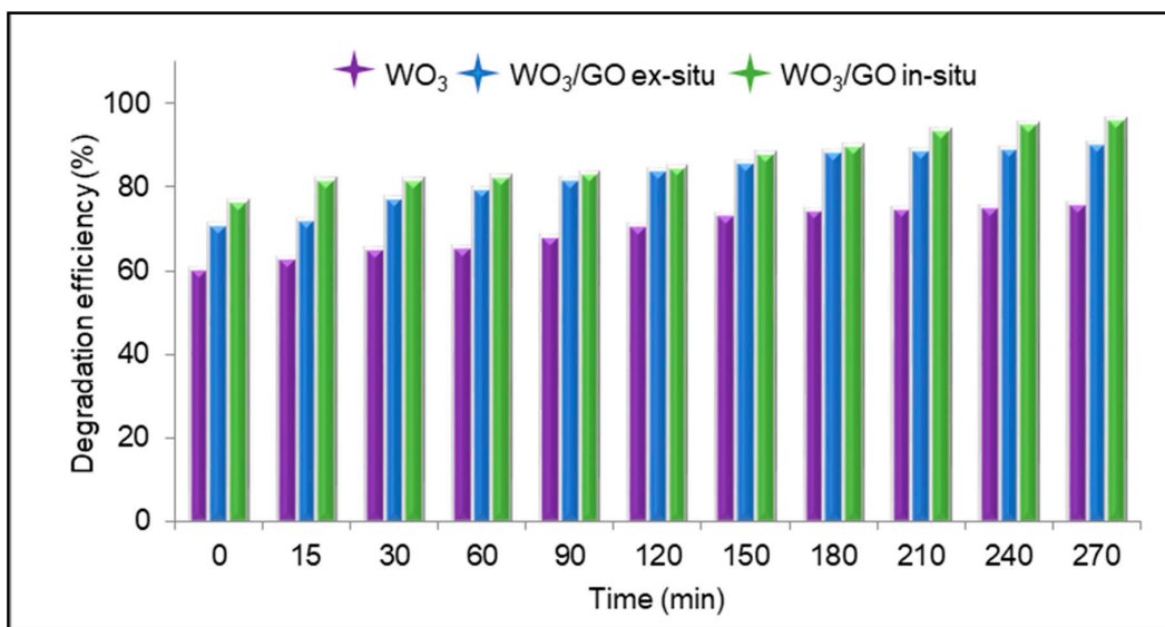
Figure 8. Degradation efficiency of MB.
