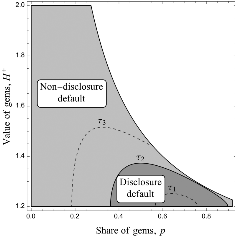
Figure 1. Optimal default rule (with L = 0.3 , L^+ = 0.6 , H = 1.2 , \tau_1 = 0.275 , \tau_2 = 0.285 , \tau_3 = 0.295 , and c \sim U[0, 1] ). Outside the gray areas, Assumption 1 is not satisfied.
