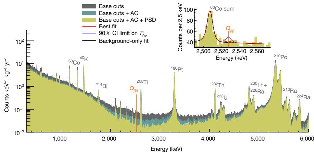
Fig. 4 | Physics spectrum for 1,038.4 kg yr of TeO 2 exposure. We separately show the effects of the base cuts, the anti-coincidence (AC) cut, and the pulse shape discrimination (PSD). The most prominent background peaks in the
