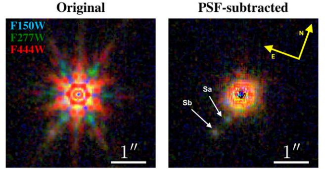
Figure 8. The left panel shows the combined multicolour image from the raw NIRCam image filters F150W, F277W, and F444W and the right panel shows the corresponding PSF-subtracted image where the two companions, Sa and Sb, are clearly visible.
