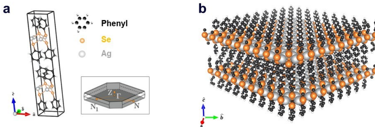
Figure 1. Silver benzeneselenolate ( [AgSePh]_\infty ) unit cell and molecular structure. a, Primitive cell and first Brillouin zone (inset); see SI for cell coordinates. b, Extended layered molecular structure of [AgSePh]_\infty consisting of 2D sheets of AgSe spaced by phenyl groups.
