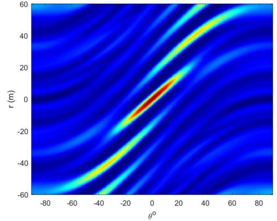
Fig. 3. Beam pattern in the (r, \theta) space for a log-FDA of 8 elements, with f_0 equal to 2.45 GHz and \Delta f equal to 10 MHz.
