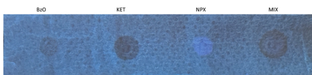
Fig. 7 Strip-test of L1 with addition of naproxen, ketoprofen, benzoate and three guests mixed (illumination at 360 nm).
