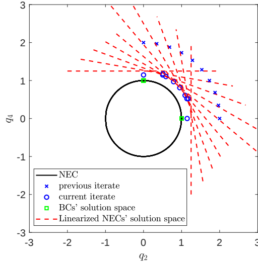
Fig. 1 First iteration with standard sequential convex programming in the presence of a nonlinear equality constraint: the linearized equality constraints do not admit the required boundary conditions.
