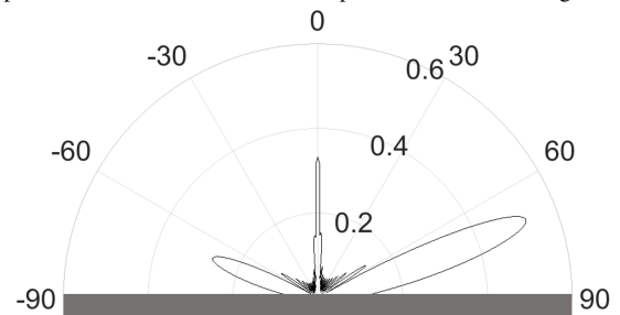
Fig. 7. Radiation pattern of the lossless anomalous reflector in [20]. Setup: normal incidence and the desired angle of reflection is 70 degrees.
