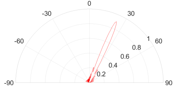
Fig. 9. Far-field radiation pattern ( \rho = 0 , S = 0 , m = 0.97 ) corresponding to the lossy phase-gradient metasurface reported in [33, Fig 2.c]. The corresponding benchmark radiation pattern is available in [33, Fig 2.d].
