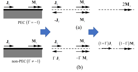
Fig. A1. Conventional (a) and modified (b) method of image currents. The image currents replace the presence of the object (scatterer, i.e., the RIS) for the purpose of calculating the field outside of it.
