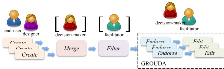
Figure 3: Methodological framework
