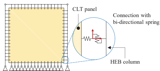
Figure 7. Numerical model of the base unit - HyST-LaR system.
