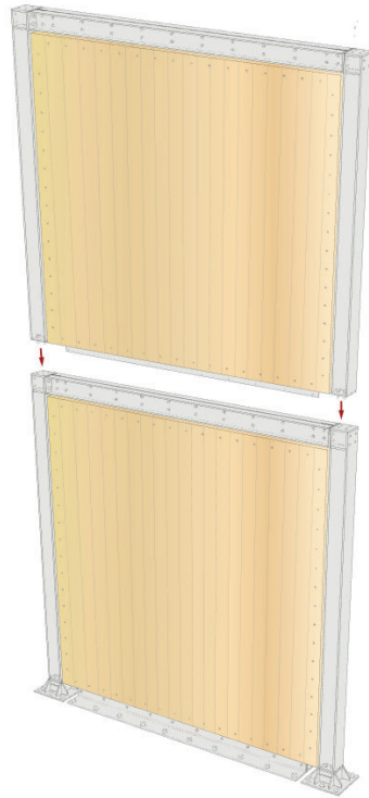
Figure 3. HyST-LaR system assembly procedure.
