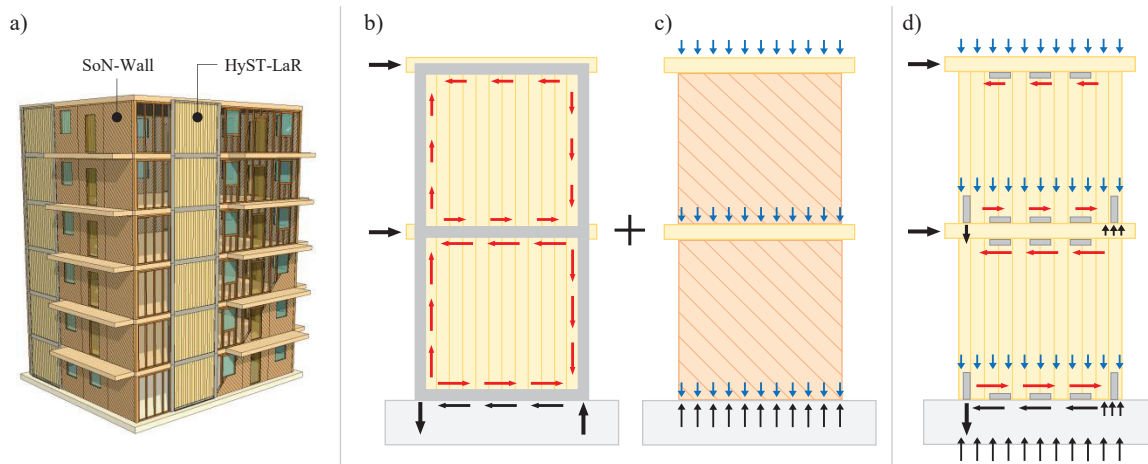
Figure 1. HyWood4Building hybrid structural system concept (a), main force distribution within HyST-LaR system (b) and SoN-Wall system (c). Force distribution of typical CLT plat-form type buildings (d).
