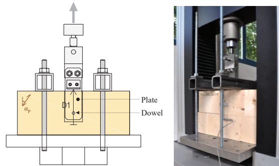
Figure 4. Set-up adopted for component-level testing.
