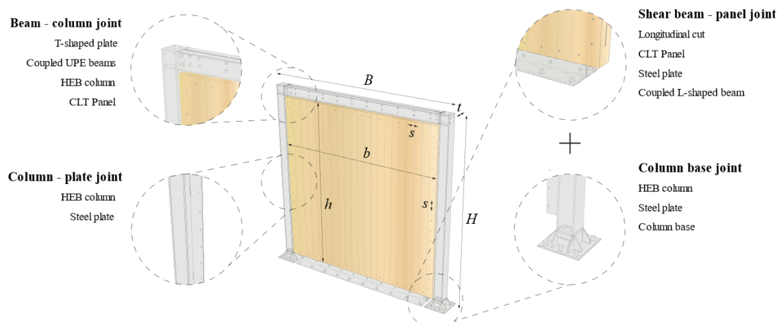
Figure 2. Base module of HyST-LaR system.
