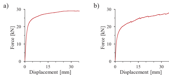
Figure 5. Mean load-slip curves from experimental testing on dowel connection of HyST-LaR system with 0^\circ (a) and 90^\circ (b) angle between the applied load and the grain of the CLT panel.
