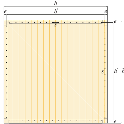
Figure 6. Geometric dimensions for the analytical model of HyST-LAR module.
