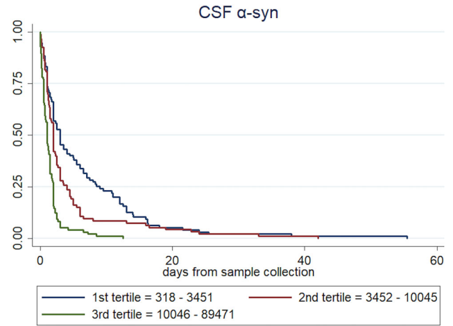
FIGURE 2 Prognostic value of CSF \alpha -syn. Survival curve in patients of the whole prion cohort according to the values of CSF \alpha -synuclein. \alpha -syn, alpha-synuclein; CSF, cerebrospinal fluid
