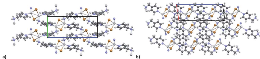
Fig. 7 (a) Packing along the a -axis; (b) packing along the b -axis. Cell axis colour: a is red, b is green and c is blue.
