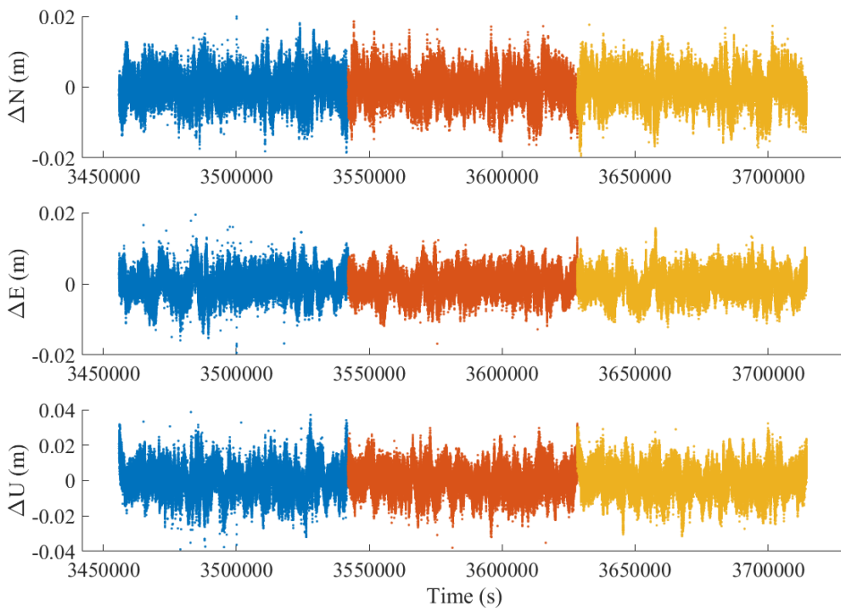
Figure 6 1 Hz time series of three days; every color represents a different day.
