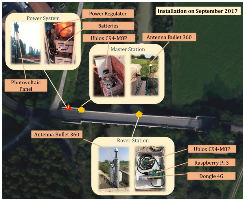
53 Figure 3 Layout of the GNSS monitoring system installed on the bridge. 54
