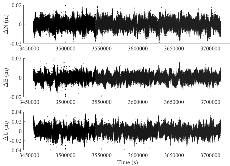
Figure 4 Three days 1 Hz time series produced from u-blox C94-M8P RTK embedded module.
