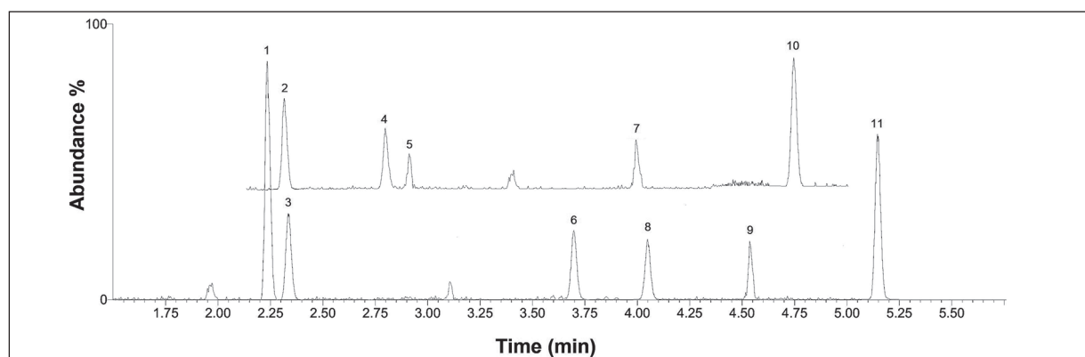
Figure 1. UHPLC-MS/MS chromatogram of urine sample fortified with the analytes at 0.01 µg/L and their ISs. 1, acetyl norfentanyl-D5 (A-D5); 2, cis-3-methylnorfentanyl; 3, trans-3-methylnorfentanyl; 4, norsufentani; 5, ofentani; 6, para-fluoro furanyl fentany; 7, isobutyryl fentany; 8, phenyl fentany; 9, beta-phenyl fentany; 10, fentany-D5 (F-D5); 11, sufentani.
