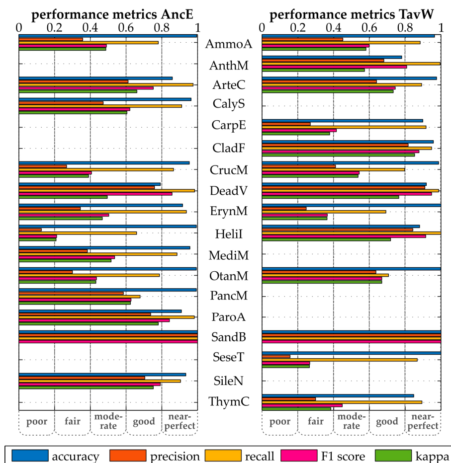
Figure A6. Performance indicators for the RFR application using WV2 data, determined from individual binary confusion matrices for each class (see Figure A5): accuracy, precision, recall, F1 score, and Cohen's kappa, calculated through Equations (A1)–(A5).
