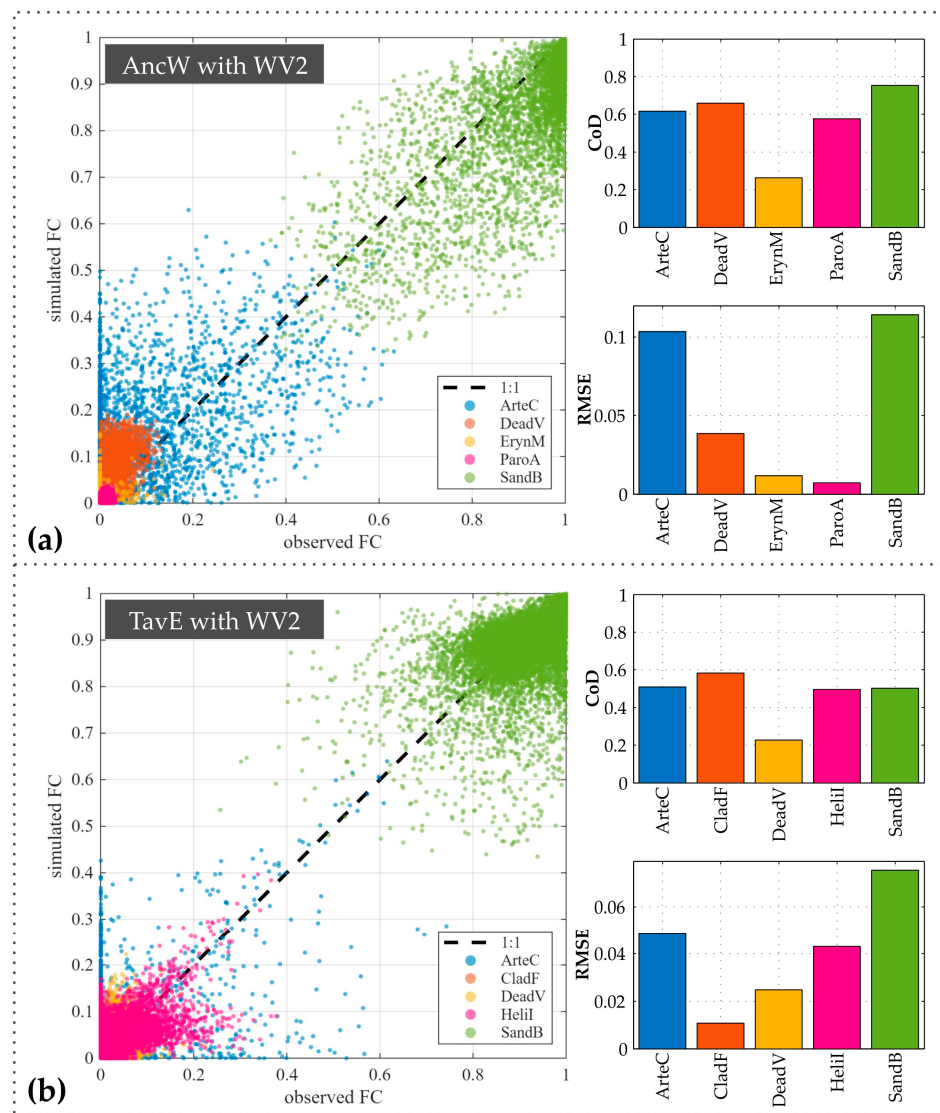
Figure 9. RFR results using unseen WV data from the plots of AncW (a) and TavE (b): scatterplots of observed versus simulated FC and bar plots of CoD and RMSE for classes that showed reasonable skill in AncE and TavW ( \text{CoD} \geq 0.3 for N_{\text{features}} = 8 in Table 4).
