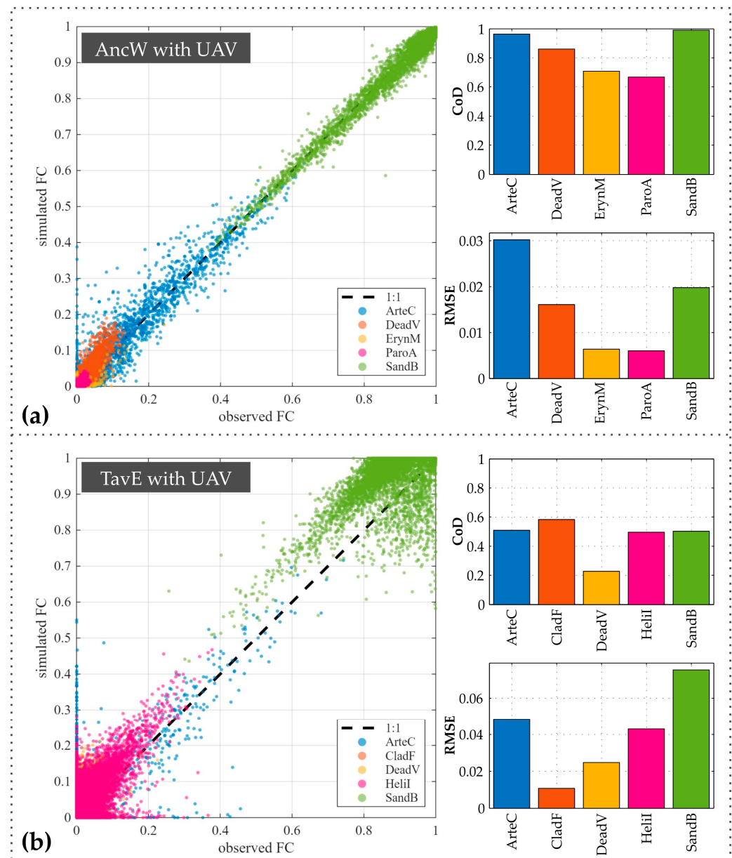
Figure 7. RFR results using unseen UAV data from the plots of AncW (a) and TavE (b): scatterplots of observed versus simulated FC and bar plots of CoD and RMSE for classes that showed reasonable skill in AncE and TavW ( \text{CoD} \geq 0.3 for N_{\text{features}} = 5 in Table 3).
