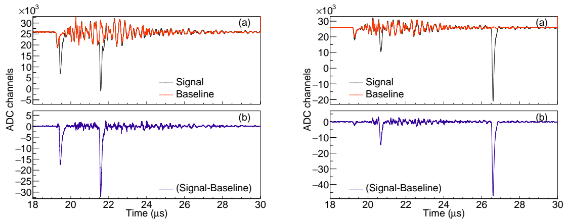
Figure 8. Two signals (frames of 12\ \mu\text{s} ) recorded for the target U1 of the PPFC. Panel (a) shows the raw signal, with the gamma flash arriving with a timestamp of about 19.2\ \mu\text{s} , followed by the ringing noise, which is overlapping to the detector signals. Panel (b) shows the result of the baseline subtraction: the gamma flash is suppressed, and the noise under the two signals is strongly reduced.
