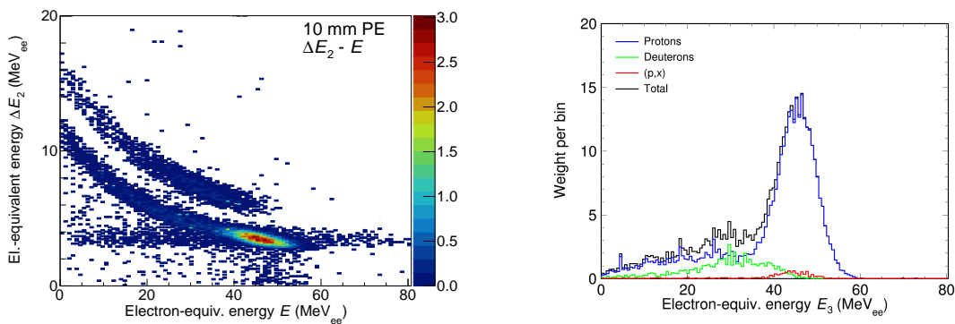
Figure 16. Simulated \Delta E_2 - E event distribution (left) panel and pulse-height distribution in the E detector (right panel) for a 2 mm-5 mm-75 mm RPT and a 10 mm polyethylene radiator. The neutron energy interval extended from 95 MeV to 105 MeV. The amount of scintillation light is measured in units of electron-equivalent energy using the non-linear light output function for organic scintillators like EJ 204.
