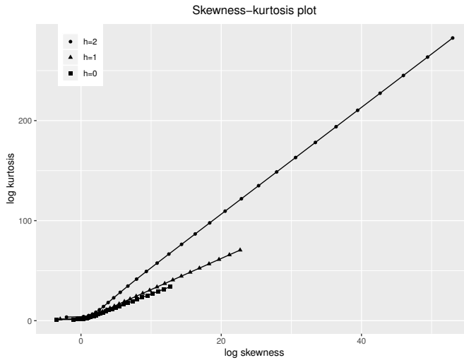
Fig. 1: Skewness-kurtosis plot (on doubly-logarithmic scale) for the g and the g -and- h distribution with a = 0 and b = 1 . The points on each curve give the skewness-kurtosis pair corresponding to increasing values of g \in \{0, 0.1, \dots, 3\} .
