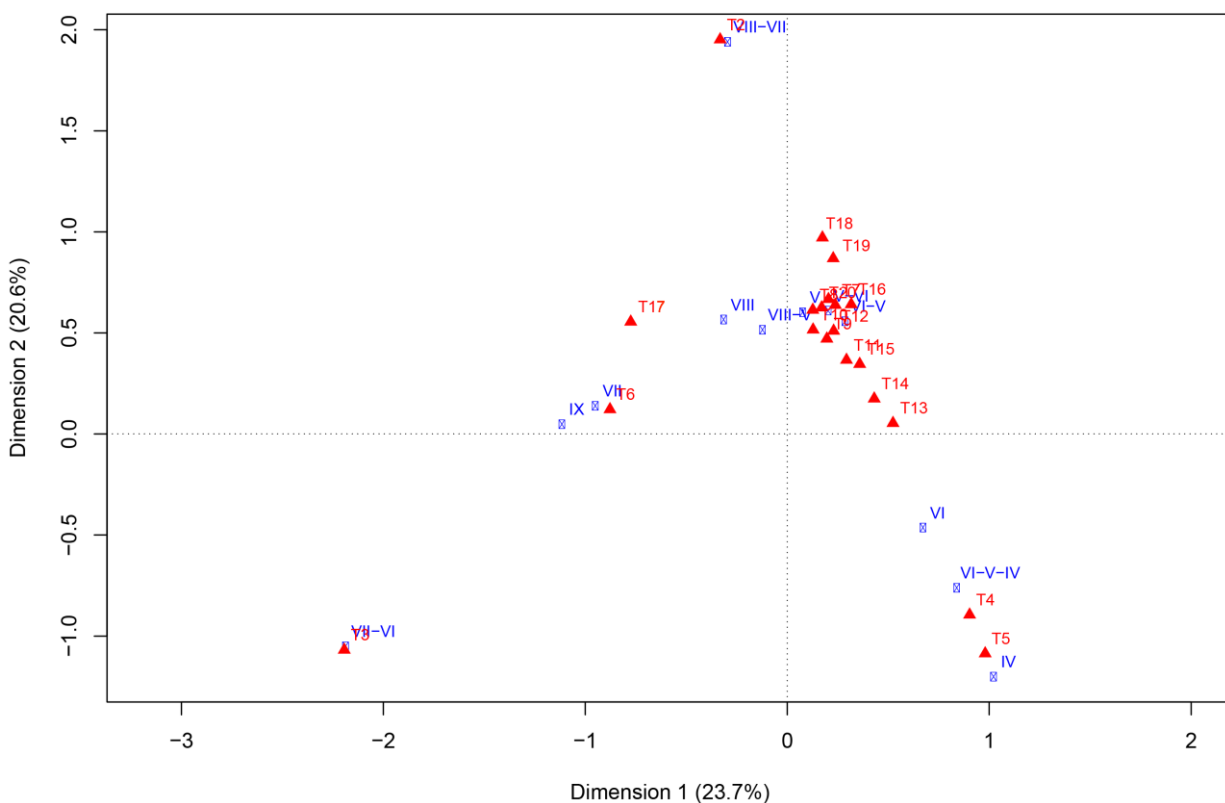
FIGURE 5 Ordination of points taxa (in red) according to chronological range (in blue) through correspondence analysis. Axes 1 and 2 describe 44.3% of the total variation.
