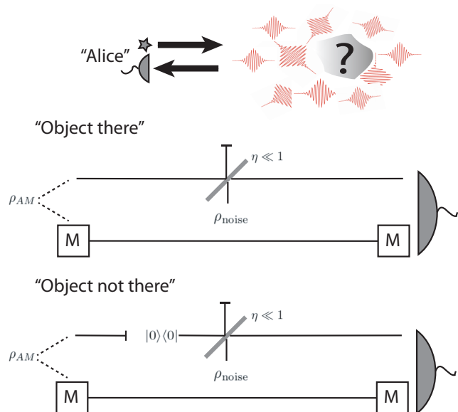
FIG. 1. The setup of quantum illumination. Alice wishes to determine whether a low-reflective target is present in a noisy environment. We model the setup as illustrated in the bottom of the figure, where Alice creates an arbitrary quantum state storing one part in a noise free memory and sending the other part as a signal. The presence of the target can be modeled as a low transmission ( \eta \ll 1 ) beam-splitter with the signal and a strong thermal state as input while the absence of the target corresponds to replacing the signal input with the vacuum. Upon discarding the non-detected modes, the beam-splitter with thermal noise corresponds to a noisy quantum Gaussian attenuator.
