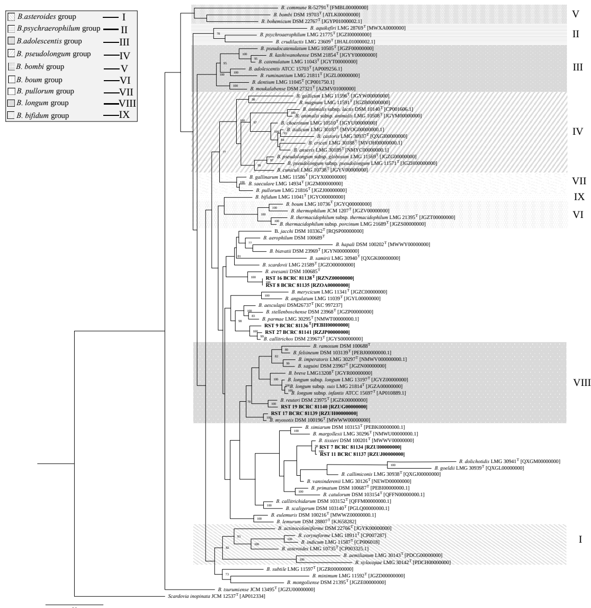
Figure 2. Phylogenetic tree based on the concatenation of proteins sequences deduced from the housekeeping genes hsp60 , rpoB , clpC , dnaJ and dnaG , showing the phylogenetic relationships between strains isolated from Egyptian fruit bats and members of the Bifidobacterium genus. The housekeeping gene-based tree was constructed by the maximum likelihood method, with corresponding sequences of Scardovia inopinata JCM 12537 T being used as outgroup. Bootstrap percentages above 70 are shown at node points, based on 1000 replicates of the phylogenetic tree.
