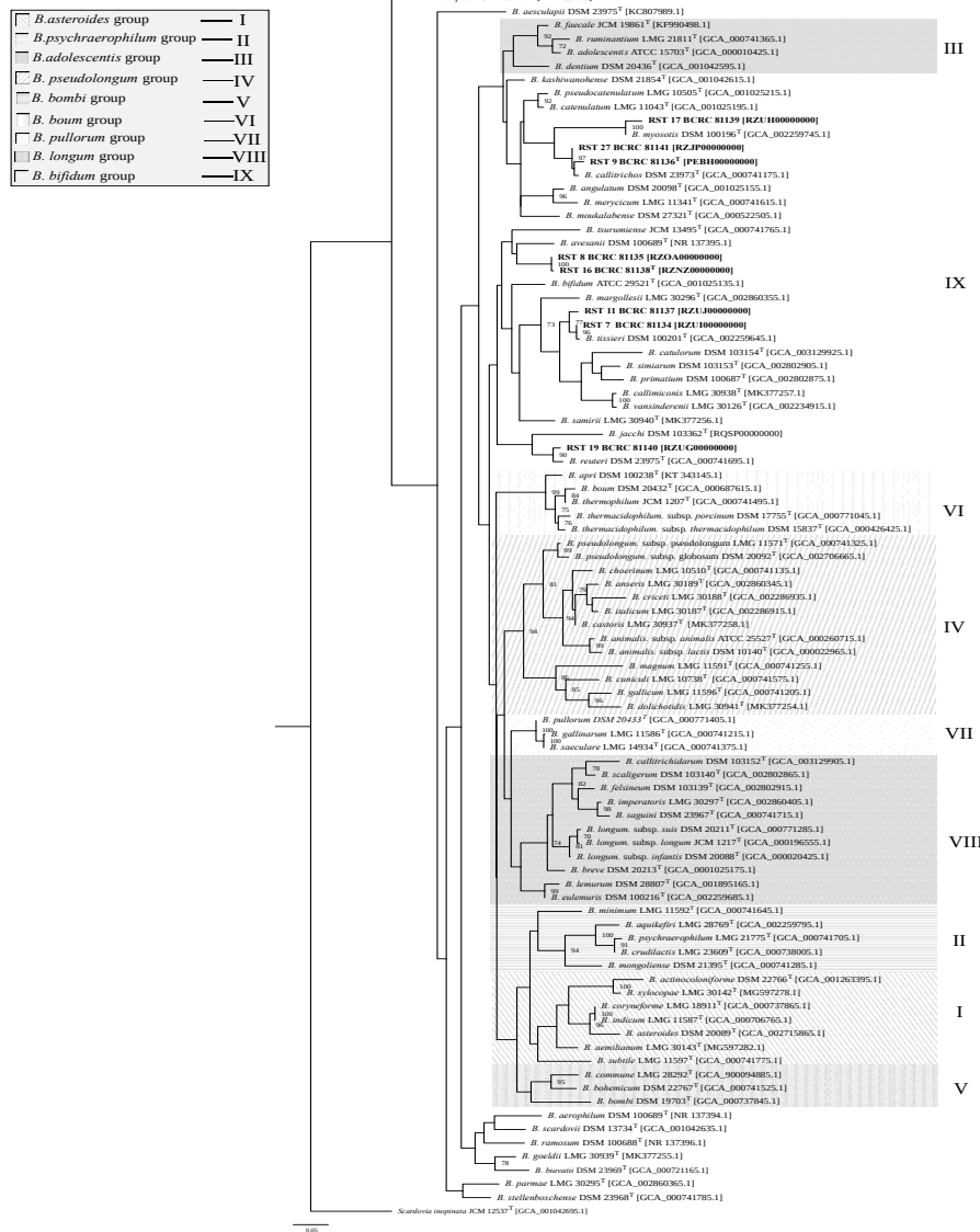
Figure 1. Phylogenetic tree of the Bifidobacterium genus based on 16S rRNA gene sequences, showing the relationship between strains isolated from Egyptian fruit bats and other members of the Bifidobacterium genus. The 16S rRNA gene-based tree was constructed by the maximum likelihood method; the corresponding sequence of Scardovia inopinata JCM 12537 T was used as outgroup. Bootstrap percentages above 70 are shown at node points, based on 1000 replicates of the phylogenetic tree.
