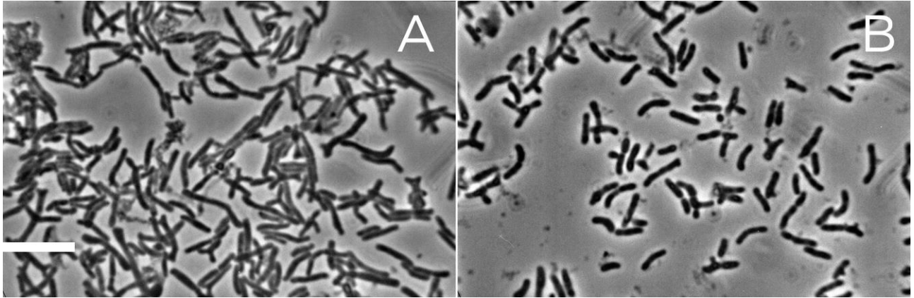
Figure 4. Phase-contrast photomicrographs of cells of B. rousetti sp. nov. RST 9 T (A) and B. vespertilionis sp. nov. RST 16 T (B) grown in TPY broth showing cellular morphology. Bar, 10 \mu m.
